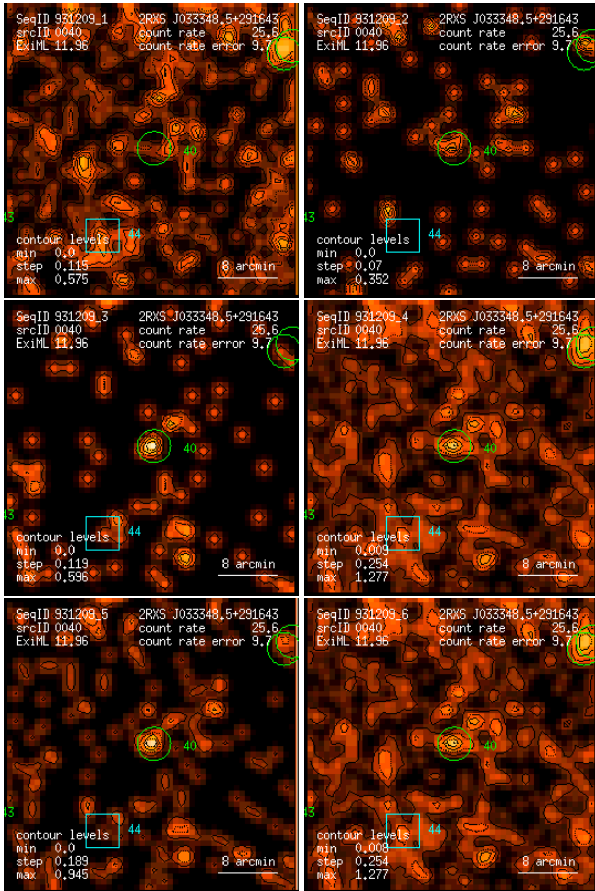
Figure 40: RASS 931209: detection 0040: band rate images, Gaussian filter: (1) PSPC channels 11 – 41, (2) 52 – 90, (3) 91 – 201, (4) 11 – 235, (5) 52 – 201, (6) 11 – 201. Broad band rates in counts/ks. Band rate contour levels in counts/ks/arcmin 2 .
