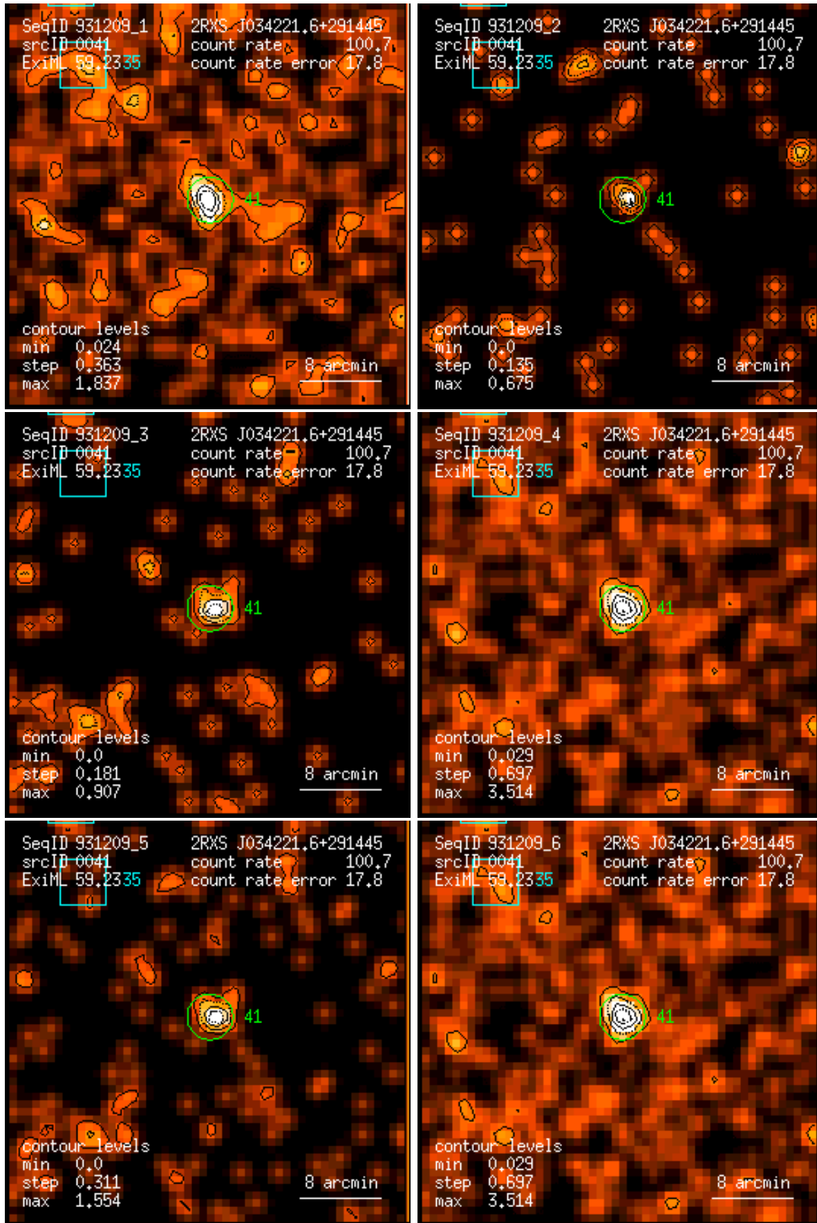
Figure 41: RASS 931209: detection 0041: band rate images, Gaussian filter: (1) PSPC channels 11 – 41, (2) 52 – 90, (3) 91 – 201, (4) 11 – 235, (5) 52 – 201, (6) 11 – 201. Broad band rates in counts/ks. Band rate contour levels in counts/ks/arcmin 2 .
