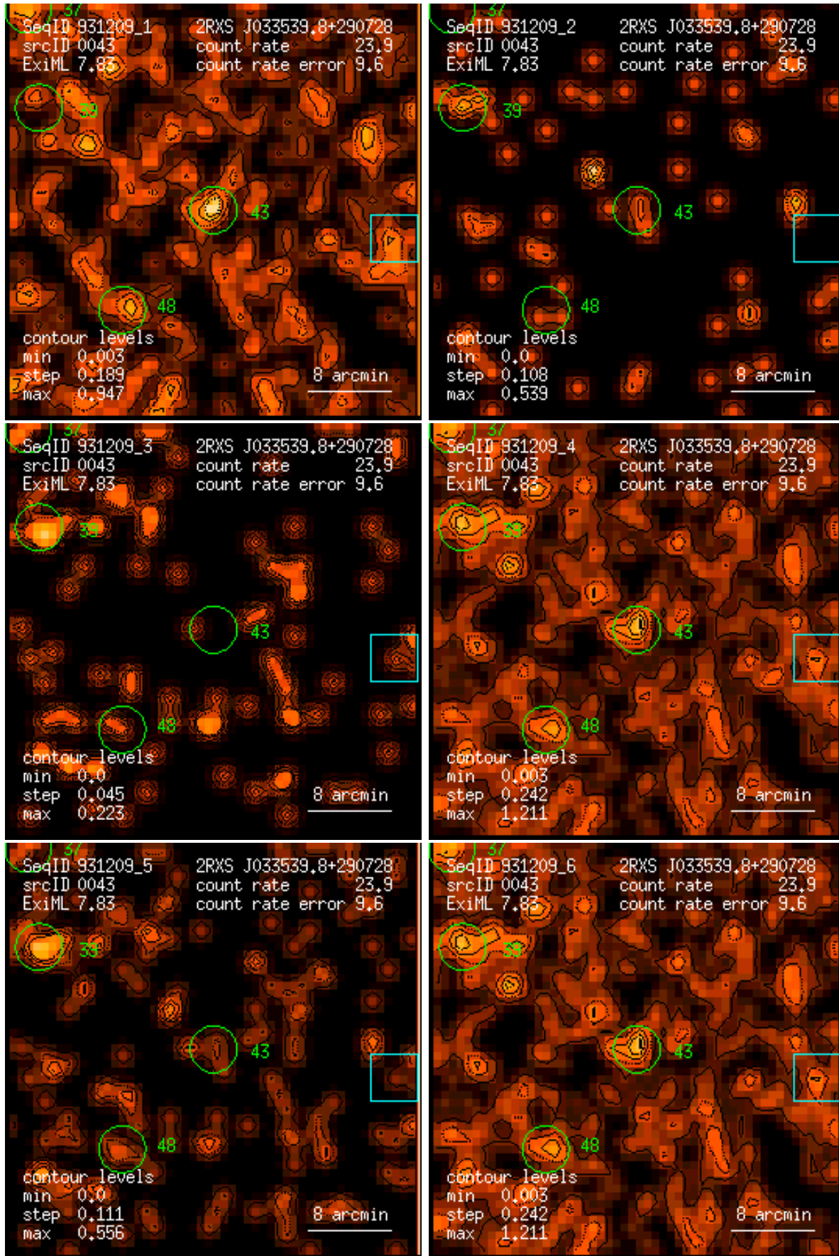
Figure 43: RASS 931209: detection 0043: band rate images, Gaussian filter: (1) PSPC channels 11 – 41, (2) 52 – 90, (3) 91 – 201, (4) 11 – 235, (5) 52 – 201, (6) 11 – 201. Broad band rates in counts/ks. Band rate contour levels in counts/ks/arcmin 2 .
