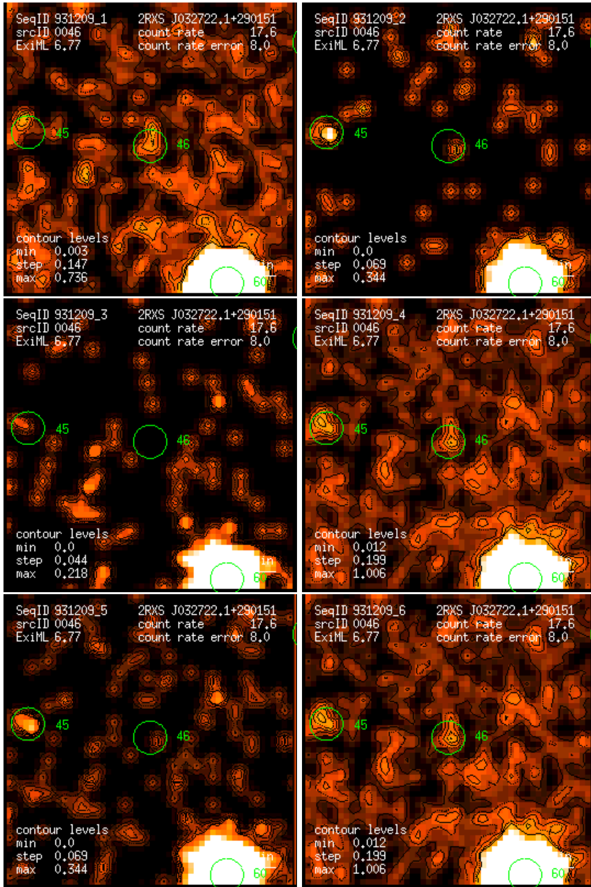
Figure 46: RASS 931209: detection 0046: band rate images, Gaussian filter: (1) PSPC channels 11 – 41, (2) 52 – 90, (3) 91 – 201, (4) 11 – 235, (5) 52 – 201, (6) 11 – 201. Broad band rates in counts/ks. Band rate contour levels in counts/ks/arcmin 2 .
