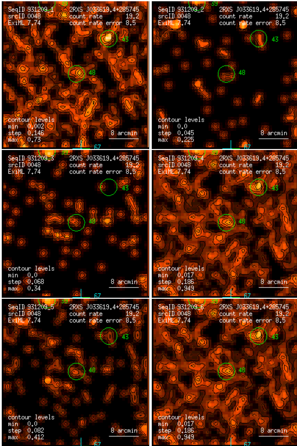
Figure 48: RASS 931209: detection 0048: band rate images, Gaussian filter: (1) PSPC channels 11 – 41, (2) 52 – 90, (3) 91 – 201, (4) 11 – 235, (5) 52 – 201, (6) 11 – 201. Broad band rates in counts/ks. Band rate contour levels in counts/ks/arcmin 2 .
