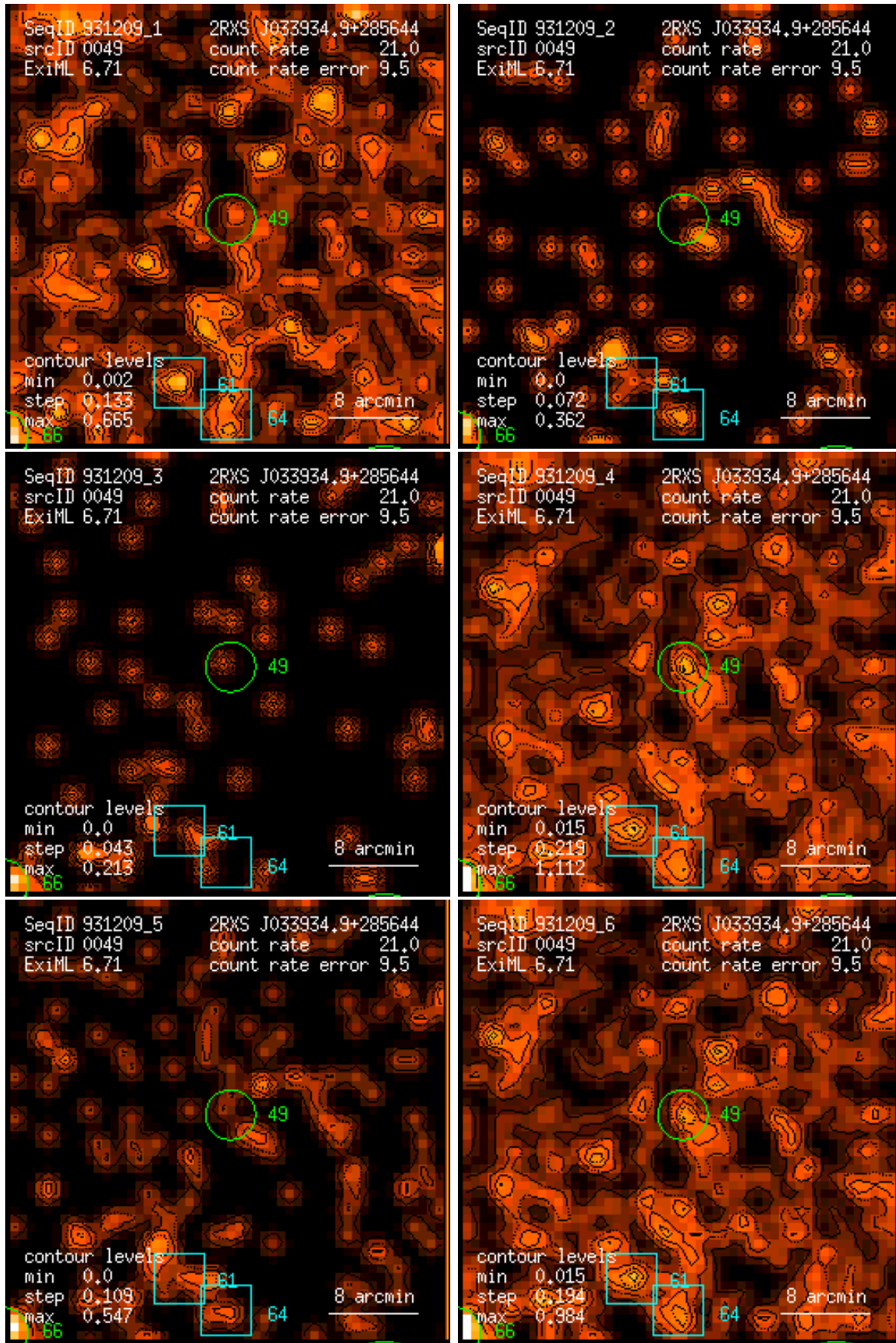
Figure 49: RASS 931209: detection 0049: band rate images, Gaussian filter: (1) PSPC channels 11 – 41, (2) 52 – 90, (3) 91 – 201, (4) 11 – 235, (5) 52 – 201, (6) 11 – 201. Broad band rates in counts/ks. Band rate contour levels in counts/ks/arcmin 2 .
