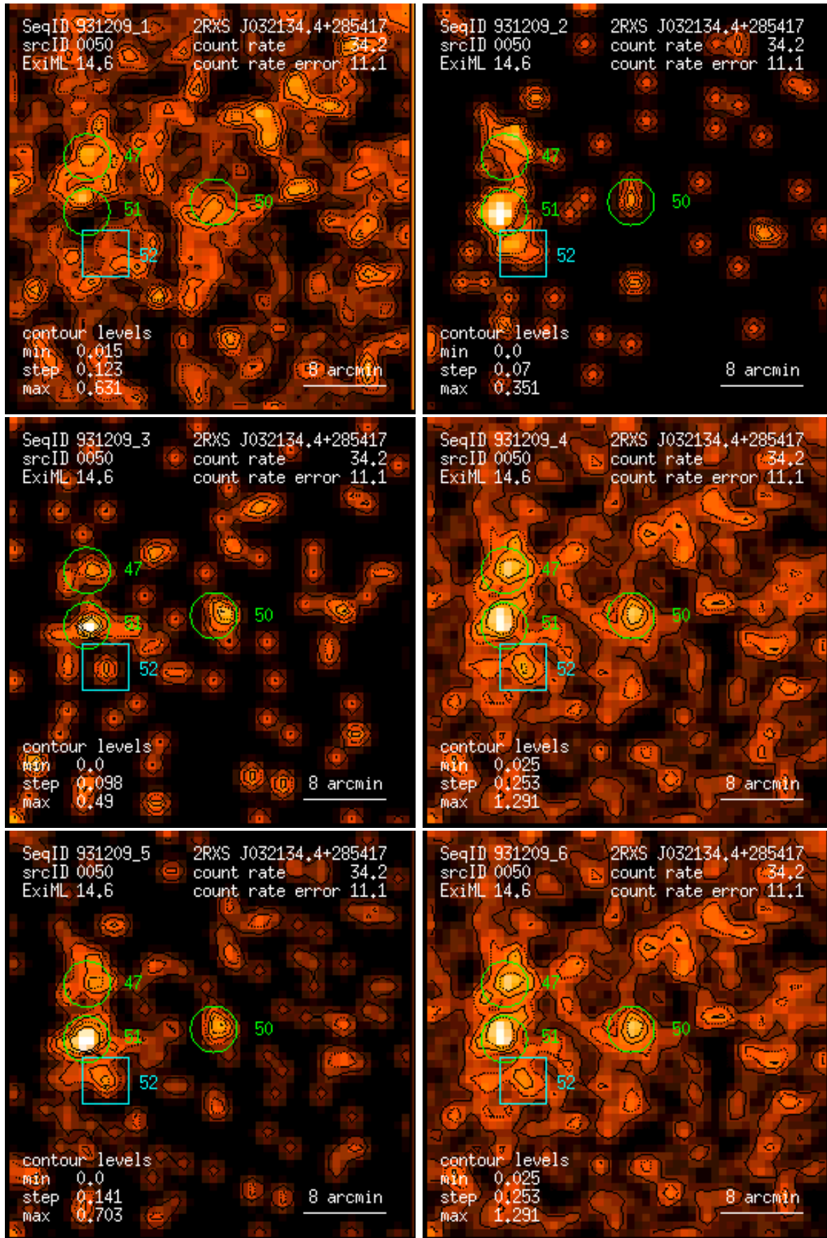
Figure 50: RASS 931209: detection 0050: band rate images, Gaussian filter: (1) PSPC channels 11 – 41, (2) 52 – 90, (3) 91 – 201, (4) 11 – 235, (5) 52 – 201, (6) 11 – 201. Broad band rates in counts/ks. Band rate contour levels in counts/ks/arcmin 2 .
