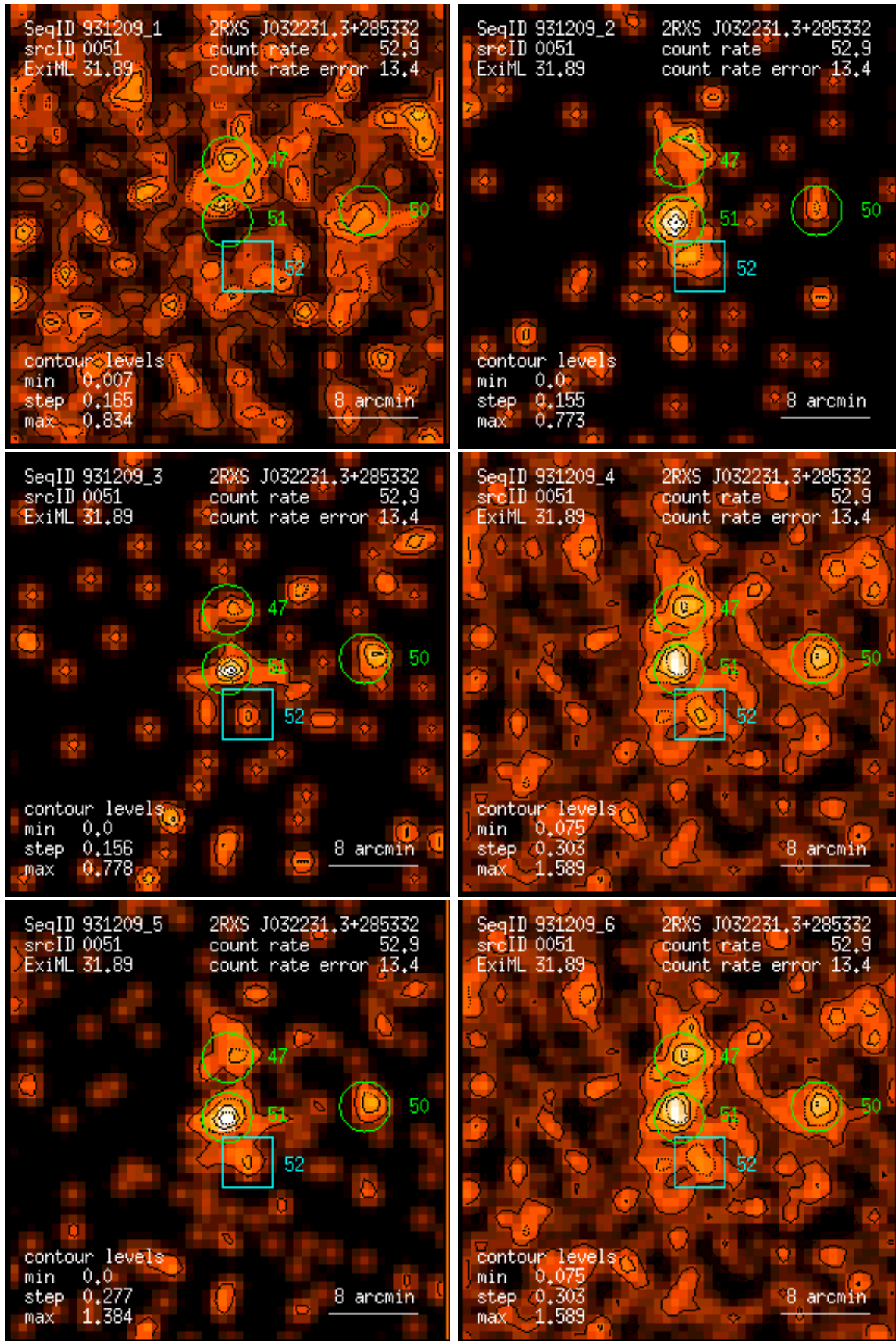
Figure 51: RASS 931209: detection 0051: band rate images, Gaussian filter: (1) PSPC channels 11 – 41, (2) 52 – 90, (3) 91 – 201, (4) 11 – 235, (5) 52 – 201, (6) 11 – 201. Broad band rates in counts/ks. Band rate contour levels in counts/ks/arcmin 2 .
