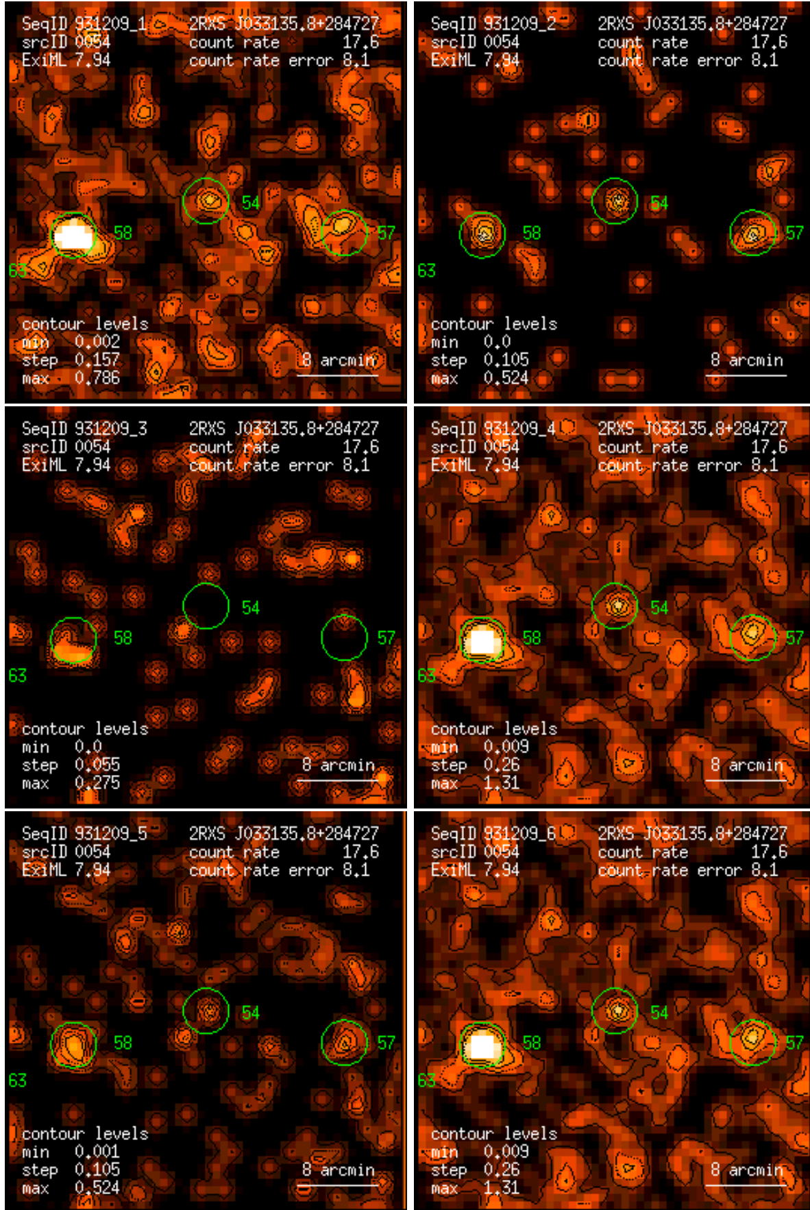
Figure 54: RASS 931209: detection 0054: band rate images, Gaussian filter: (1) PSPC channels 11 – 41, (2) 52 – 90, (3) 91 – 201, (4) 11 – 235, (5) 52 – 201, (6) 11 – 201. Broad band rates in counts/ks. Band rate contour levels in counts/ks/arcmin 2 .
