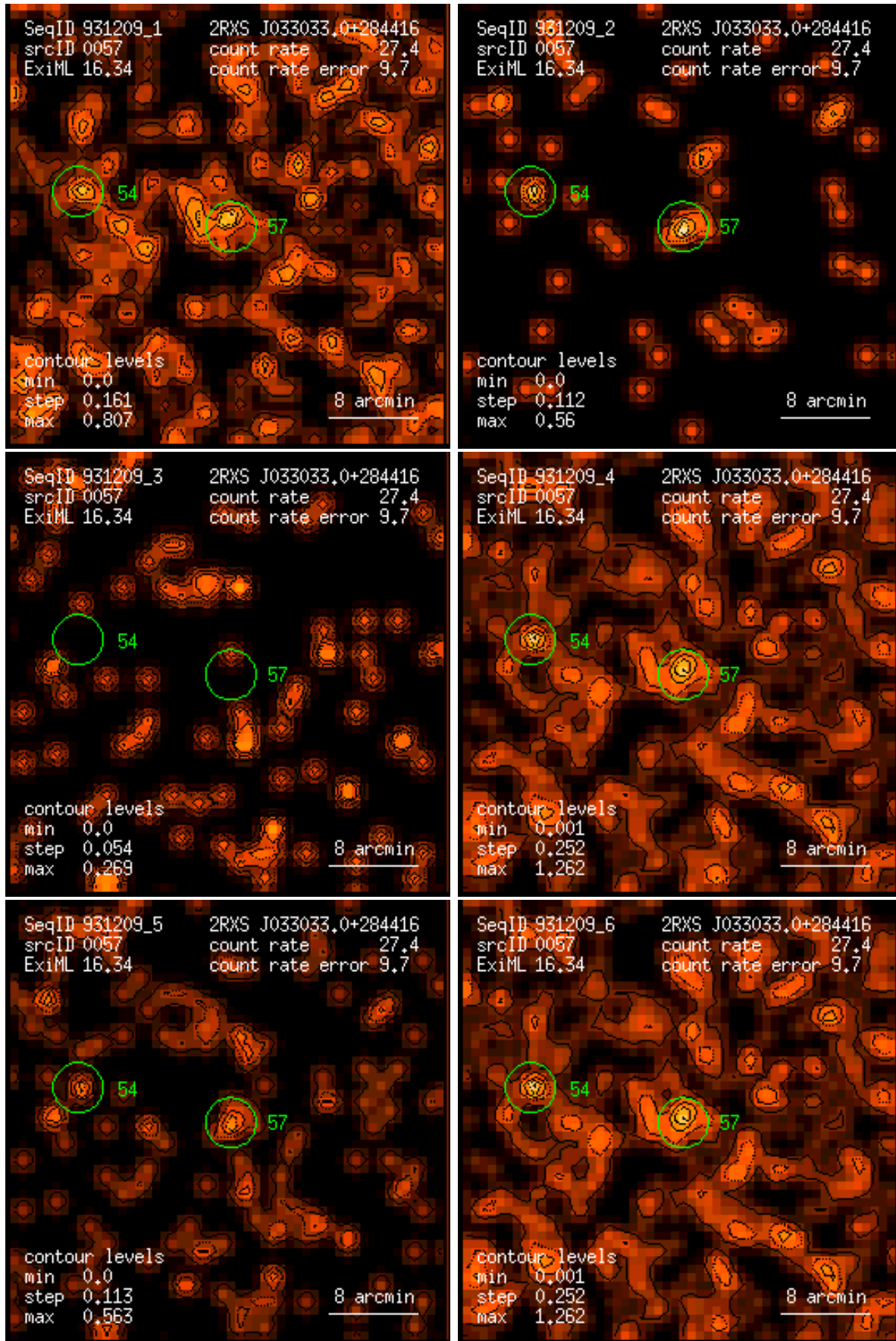
Figure 57: RASS 931209: detection 0057: band rate images, Gaussian filter: (1) PSPC channels 11 – 41, (2) 52 – 90, (3) 91 – 201, (4) 11 – 235, (5) 52 – 201, (6) 11 – 201. Broad band rates in counts/ks. Band rate contour levels in counts/ks/arcmin 2 .
