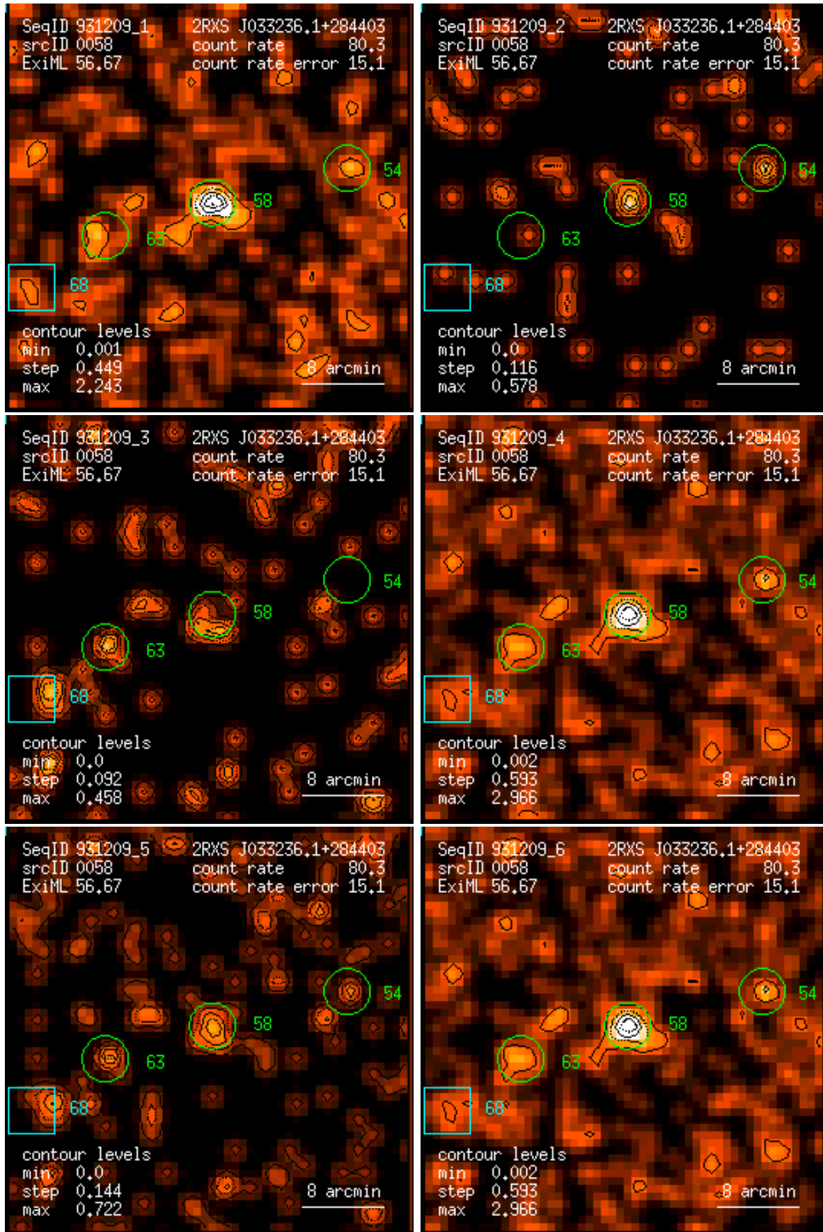
Figure 58: RASS 931209: detection 0058: band rate images, Gaussian filter: (1) PSPC channels 11 – 41, (2) 52 – 90, (3) 91 – 201, (4) 11 – 235, (5) 52 – 201, (6) 11 – 201. Broad band rates in counts/ks. Band rate contour levels in counts/ks/arcmin 2 .
