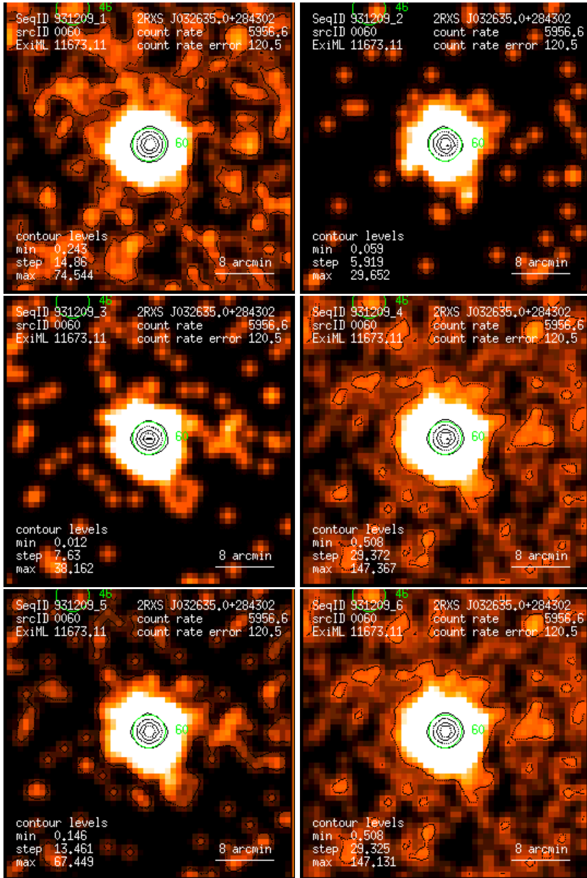
Figure 60: RASS 931209: detection 0060: band rate images, Gaussian filter: (1) PSPC channels 11 – 41, (2) 52 – 90, (3) 91 – 201, (4) 11 – 235, (5) 52 – 201, (6) 11 – 201. Broad band rates in counts/ks. Band rate contour levels in counts/ks/arcmin 2 .
