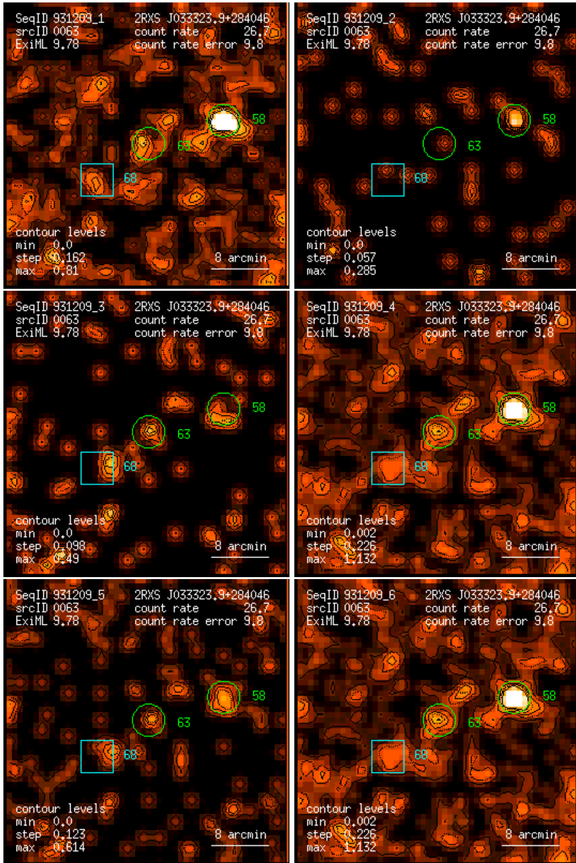
Figure 63: RASS 931209: detection 0063: band rate images, Gaussian filter: (1) PSPC channels 11 – 41, (2) 52 – 90, (3) 91 – 201, (4) 11 – 235, (5) 52 – 201, (6) 11 – 201. Broad band rates in counts/ks. Band rate contour levels in counts/ks/arcmin 2 .
