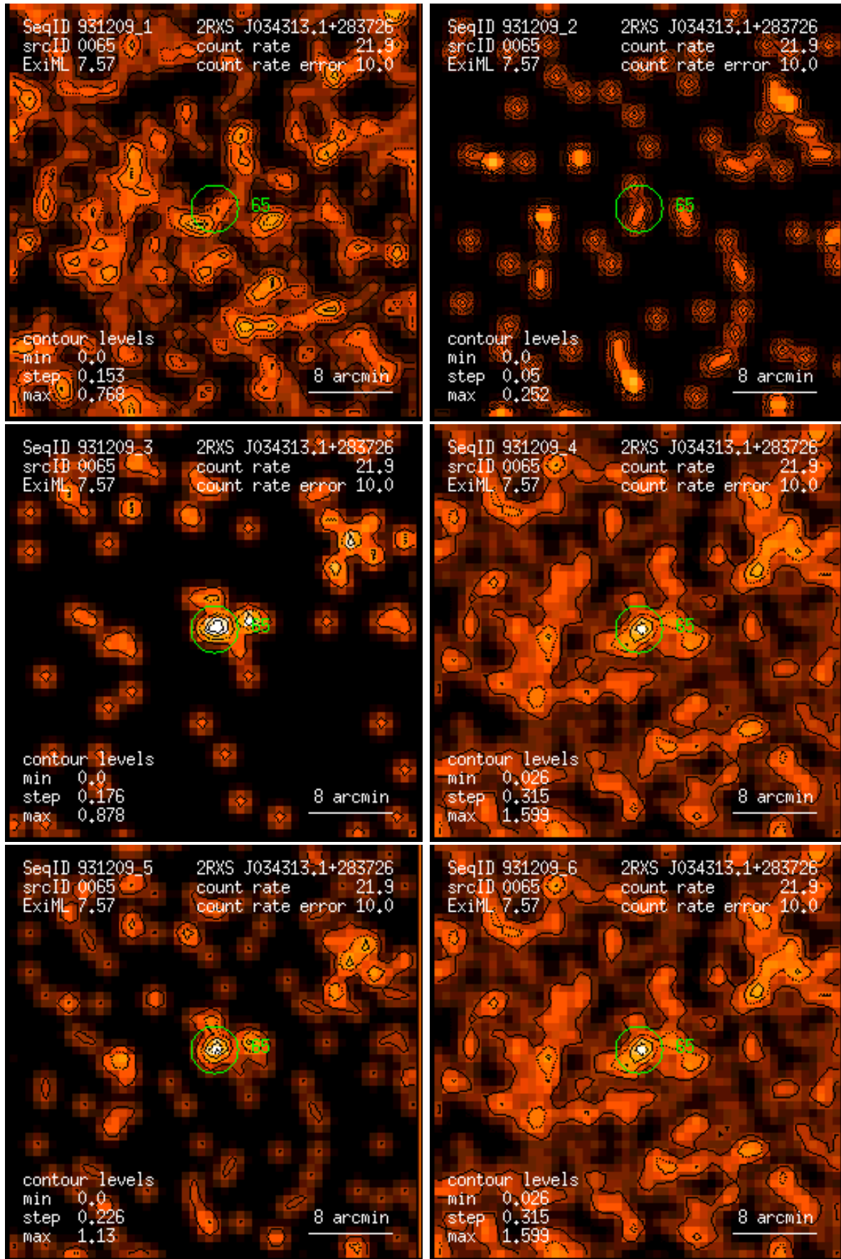
Figure 65: RASS 931209: detection 0065: band rate images, Gaussian filter: (1) PSPC channels 11 – 41, (2) 52 – 90, (3) 91 – 201, (4) 11 – 235, (5) 52 – 201, (6) 11 – 201. Broad band rates in counts/ks. Band rate contour levels in counts/ks/arcmin 2 .
