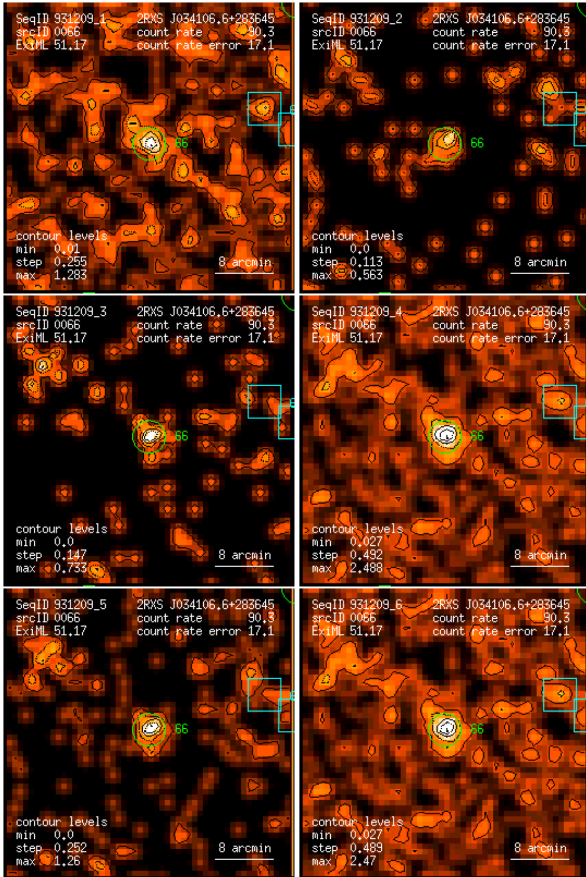
Figure 66: RASS 931209: detection 0066: band rate images, Gaussian filter: (1) PSPC channels 11 – 41, (2) 52 – 90, (3) 91 – 201, (4) 11 – 235, (5) 52 – 201, (6) 11 – 201. Broad band rates in counts/ks. Band rate contour levels in counts/ks/arcmin 2 .
