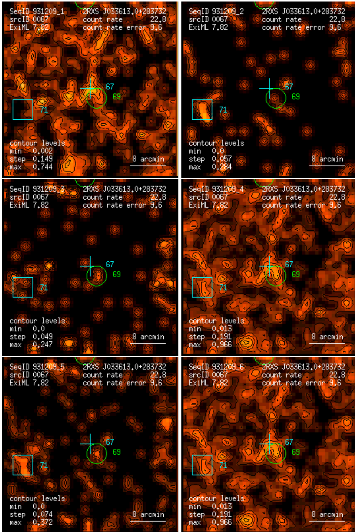
Figure 67: RASS 931209: detection 0067: band rate images, Gaussian filter: (1) PSPC channels 11 – 41, (2) 52 – 90, (3) 91 – 201, (4) 11 – 235, (5) 52 – 201, (6) 11 – 201. Broad band rates in counts/ks. Band rate contour levels in counts/ks/arcmin 2 .
