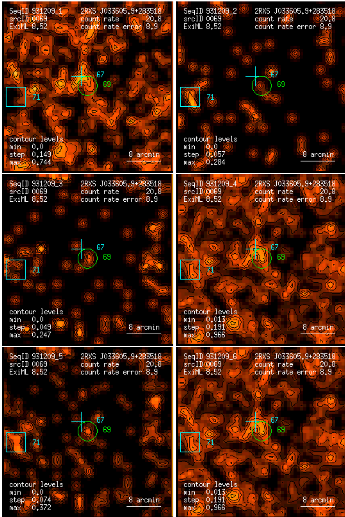
Figure 69: RASS 931209: detection 0069: band rate images, Gaussian filter: (1) PSPC channels 11 – 41, (2) 52 – 90, (3) 91 – 201, (4) 11 – 235, (5) 52 – 201, (6) 11 – 201. Broad band rates in counts/ks. Band rate contour levels in counts/ks/arcmin 2 .
