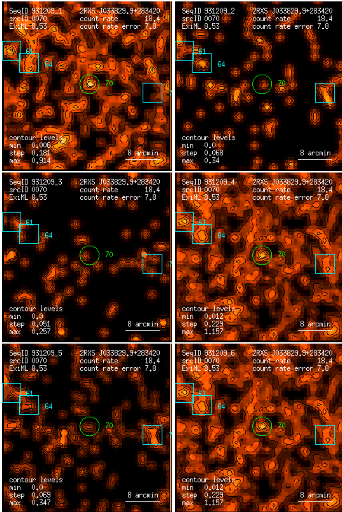
Figure 70: RASS 931209: detection 0070: band rate images, Gaussian filter: (1) PSPC channels 11 – 41, (2) 52 – 90, (3) 91 – 201, (4) 11 – 235, (5) 52 – 201, (6) 11 – 201. Broad band rates in counts/ks. Band rate contour levels in counts/ks/arcmin 2 .
