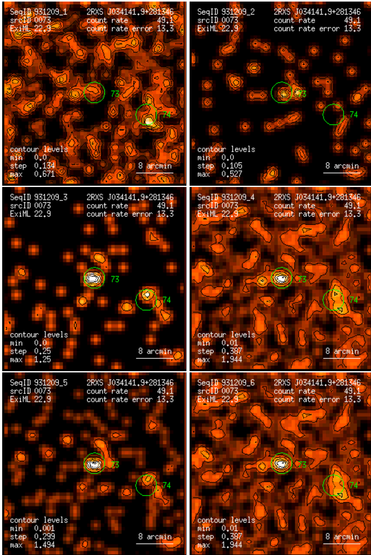
Figure 73: RASS 931209: detection 0073: band rate images, Gaussian filter: (1) PSPC channels 11 – 41, (2) 52 – 90, (3) 91 – 201, (4) 11 – 235, (5) 52 – 201, (6) 11 – 201. Broad band rates in counts/ks. Band rate contour levels in counts/ks/arcmin 2 .
