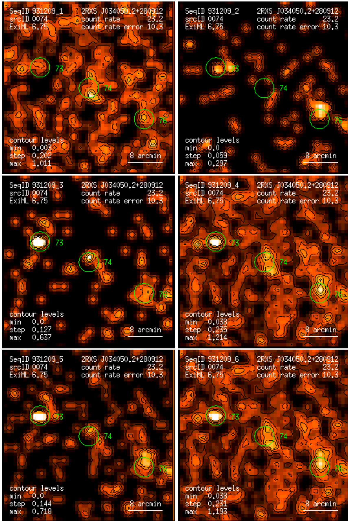
Figure 74: RASS 931209: detection 0074: band rate images, Gaussian filter: (1) PSPC channels 11 – 41, (2) 52 – 90, (3) 91 – 201, (4) 11 – 235, (5) 52 – 201, (6) 11 – 201. Broad band rates in counts/ks. Band rate contour levels in counts/ks/arcmin 2 .
