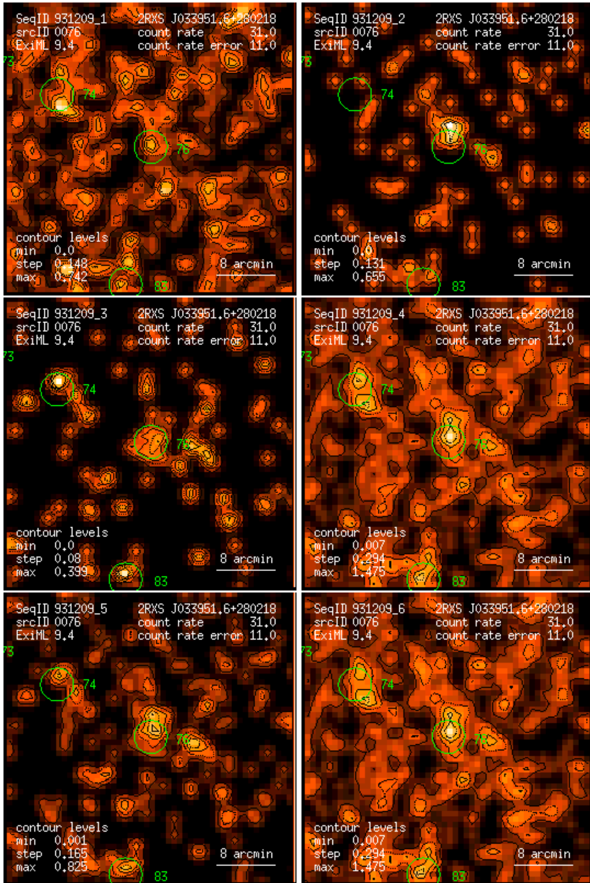
Figure 76: RASS 931209: detection 0076: band rate images, Gaussian filter: (1) PSPC channels 11 – 41, (2) 52 – 90, (3) 91 – 201, (4) 11 – 235, (5) 52 – 201, (6) 11 – 201. Broad band rates in counts/ks. Band rate contour levels in counts/ks/arcmin 2 .
