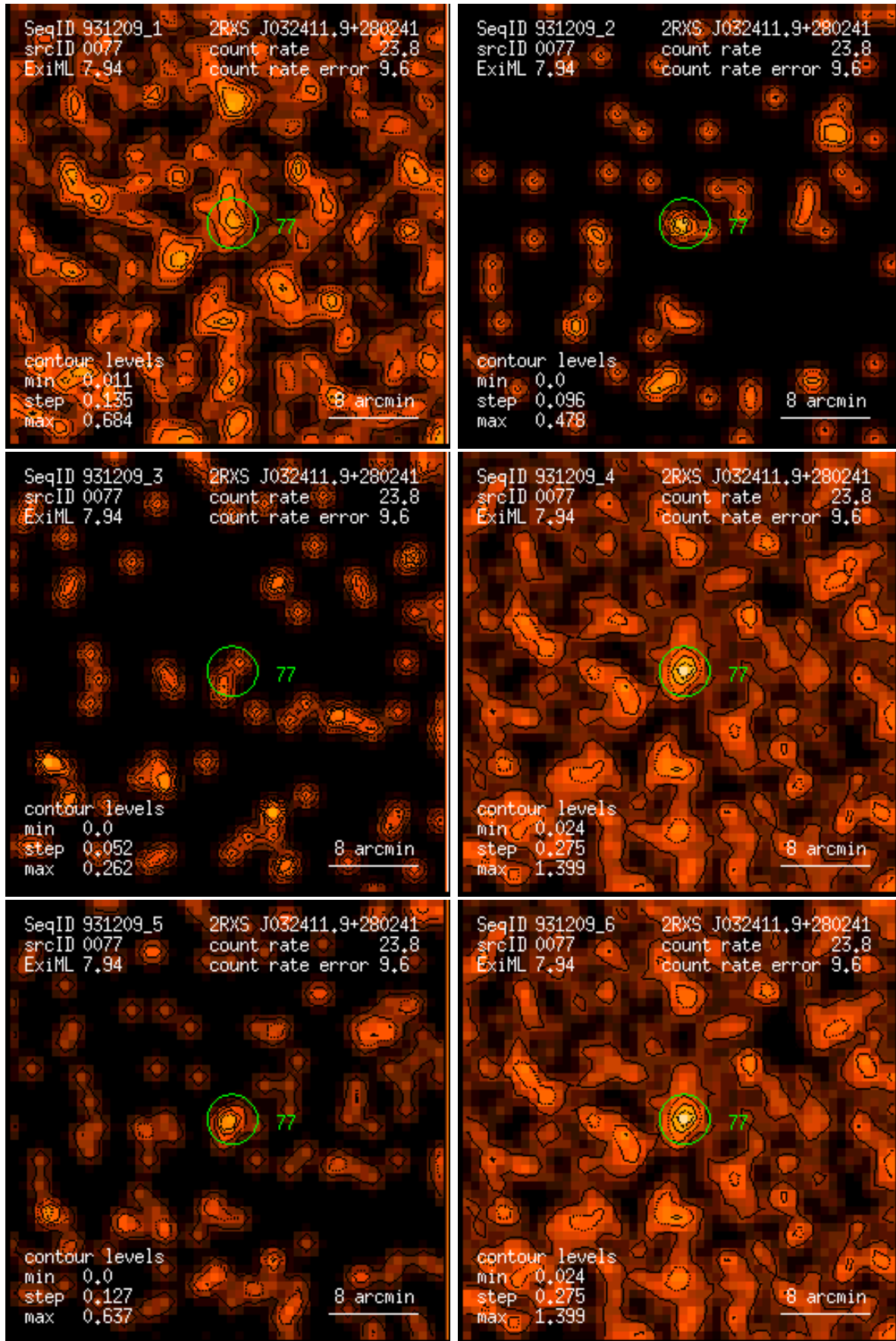
Figure 77: RASS 931209: detection 0077: band rate images, Gaussian filter: (1) PSPC channels 11 – 41, (2) 52 – 90, (3) 91 – 201, (4) 11 – 235, (5) 52 – 201, (6) 11 – 201. Broad band rates in counts/ks. Band rate contour levels in counts/ks/arcmin 2 .
