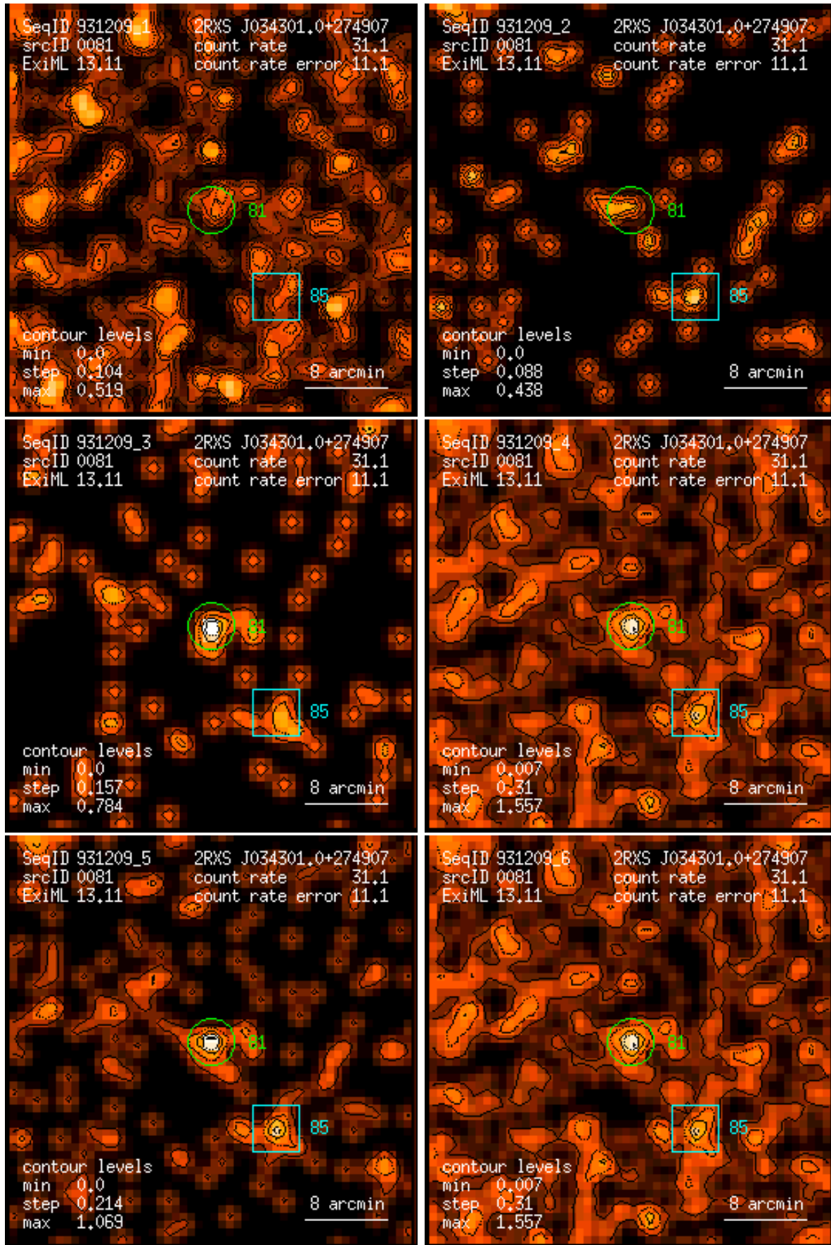
Figure 81: RASS 931209: detection 0081: band rate images, Gaussian filter: (1) PSPC channels 11 – 41, (2) 52 – 90, (3) 91 – 201, (4) 11 – 235, (5) 52 – 201, (6) 11 – 201. Broad band rates in counts/ks. Band rate contour levels in counts/ks/arcmin 2 .
