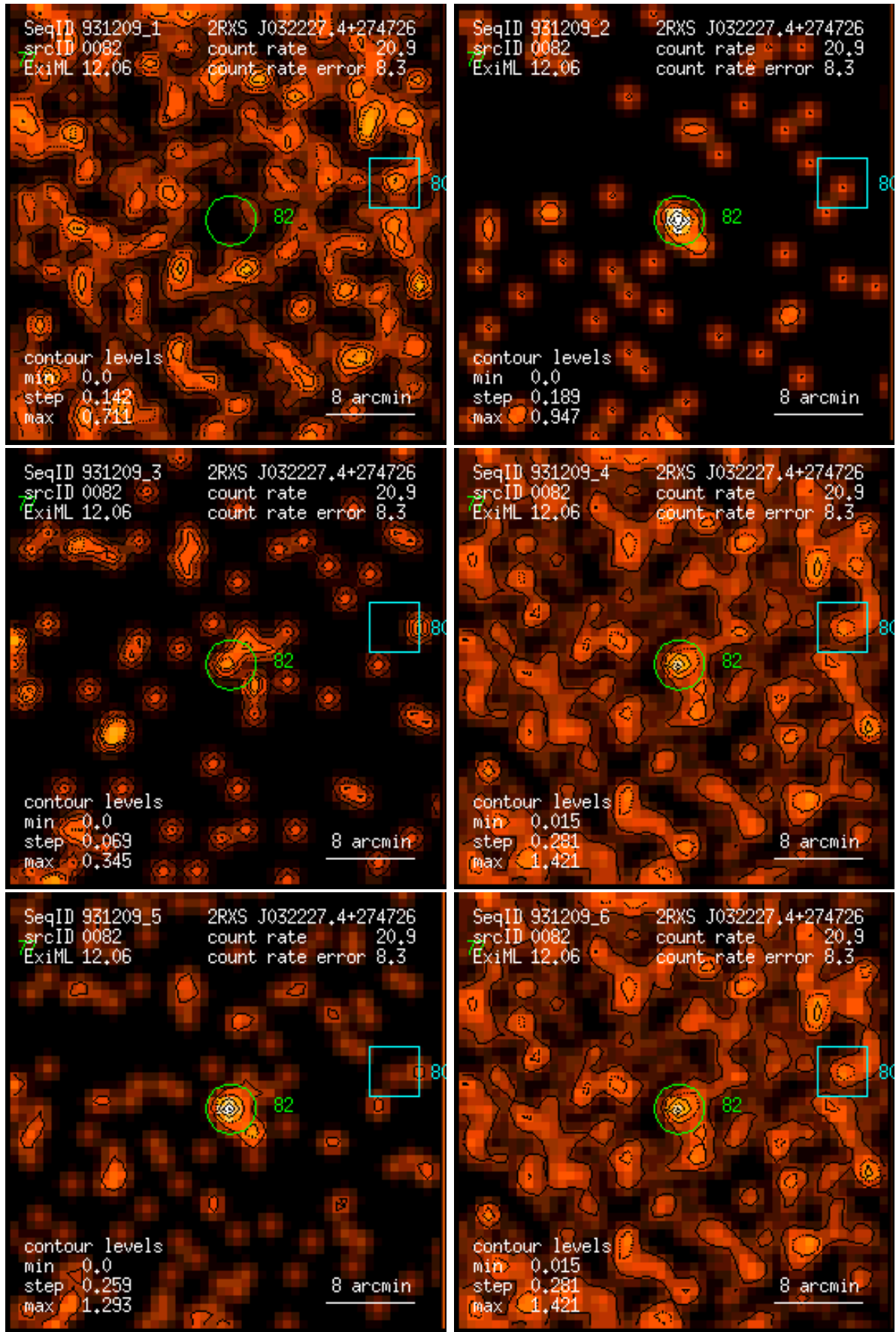
Figure 82: RASS 931209: detection 0082: band rate images, Gaussian filter: (1) PSPC channels 11 – 41, (2) 52 – 90, (3) 91 – 201, (4) 11 – 235, (5) 52 – 201, (6) 11 – 201. Broad band rates in counts/ks. Band rate contour levels in counts/ks/arcmin 2 .
