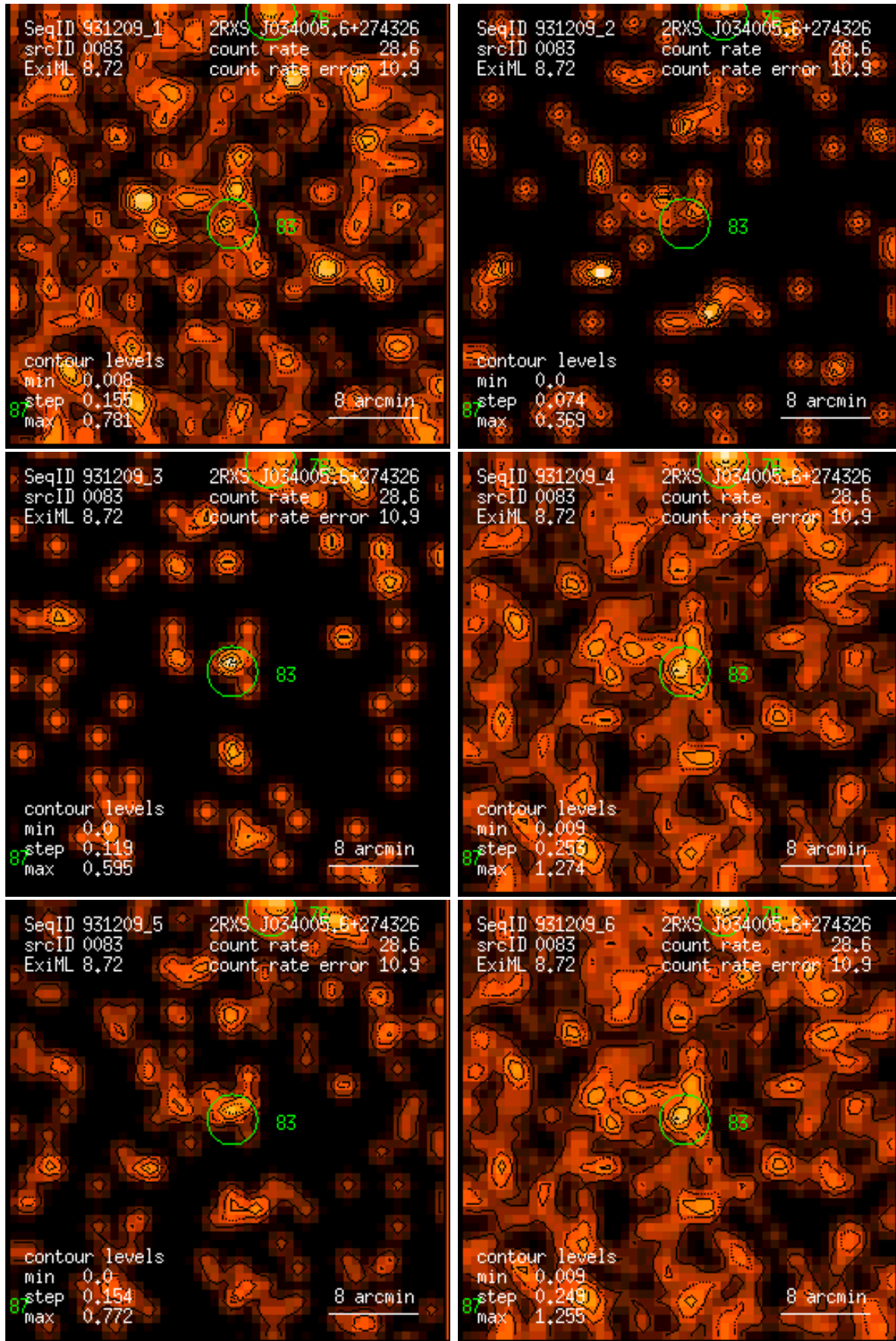
Figure 83: RASS 931209: detection 0083: band rate images, Gaussian filter: (1) PSPC channels 11 – 41, (2) 52 – 90, (3) 91 – 201, (4) 11 – 235, (5) 52 – 201, (6) 11 – 201. Broad band rates in counts/ks. Band rate contour levels in counts/ks/arcmin 2 .
