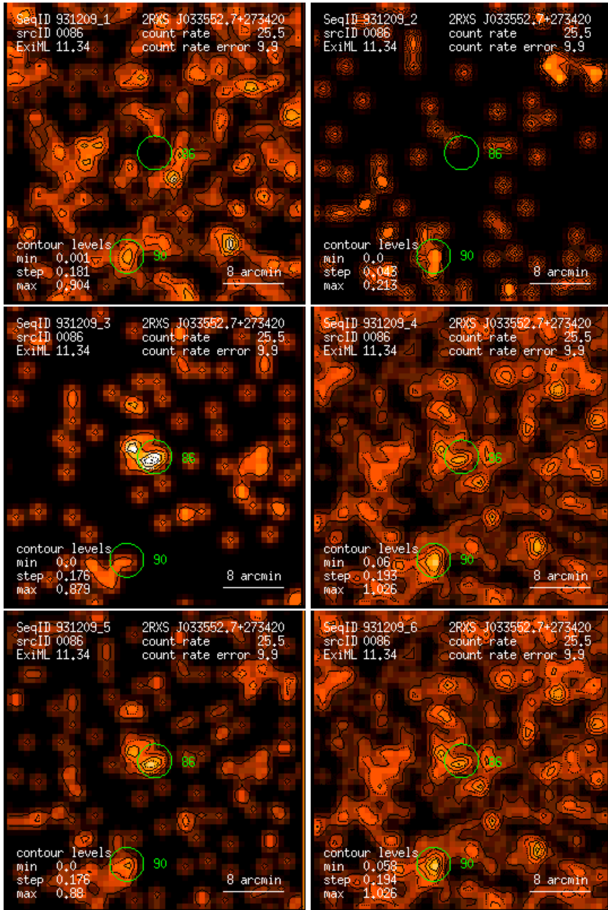
Figure 86: RASS 931209: detection 0086: band rate images, Gaussian filter: (1) PSPC channels 11 – 41, (2) 52 – 90, (3) 91 – 201, (4) 11 – 235, (5) 52 – 201, (6) 11 – 201. Broad band rates in counts/ks. Band rate contour levels in counts/ks/arcmin 2 .
