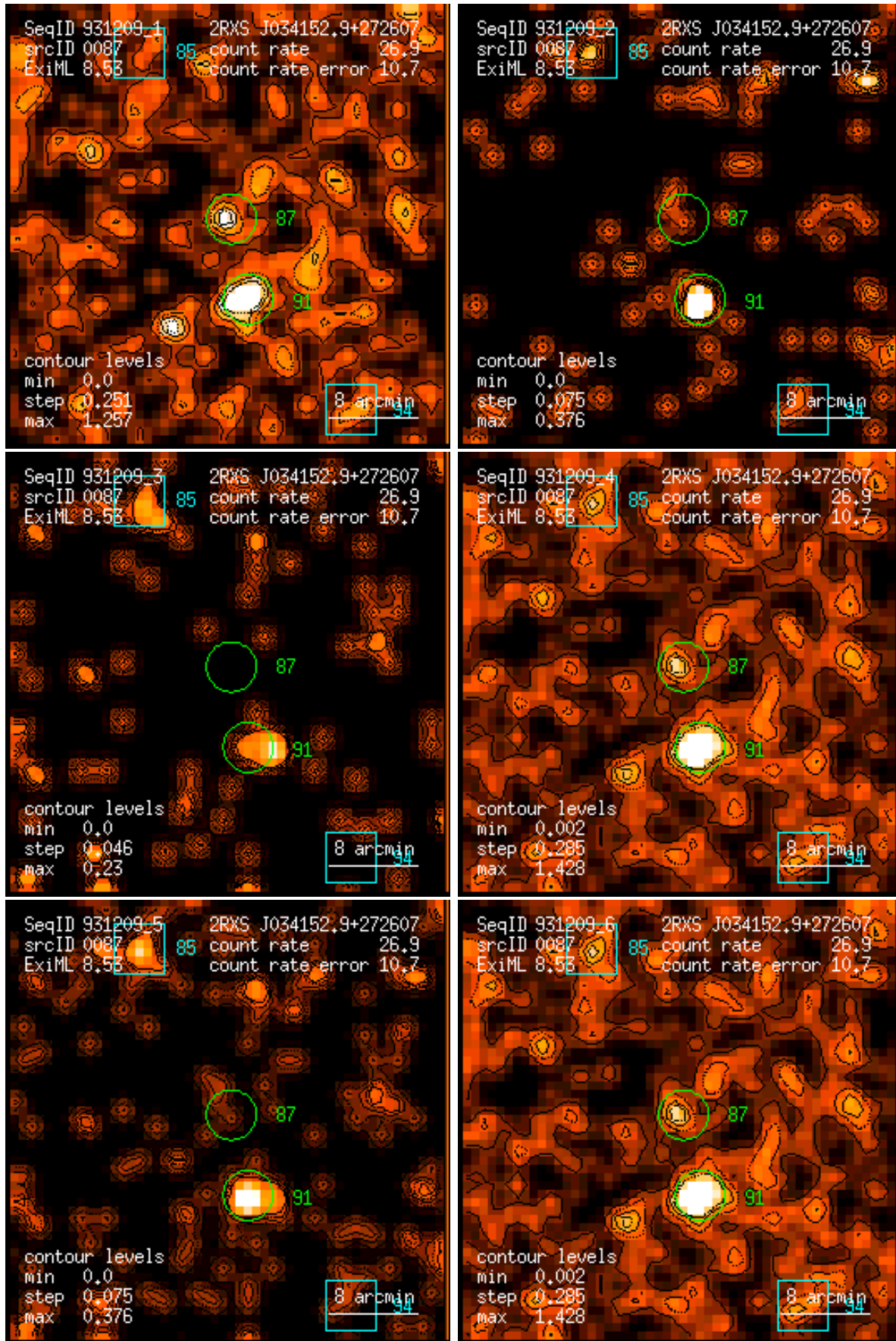
Figure 87: RASS 931209: detection 0087: band rate images, Gaussian filter: (1) PSPC channels 11 – 41, (2) 52 – 90, (3) 91 – 201, (4) 11 – 235, (5) 52 – 201, (6) 11 – 201. Broad band rates in counts/ks. Band rate contour levels in counts/ks/arcmin 2 .
