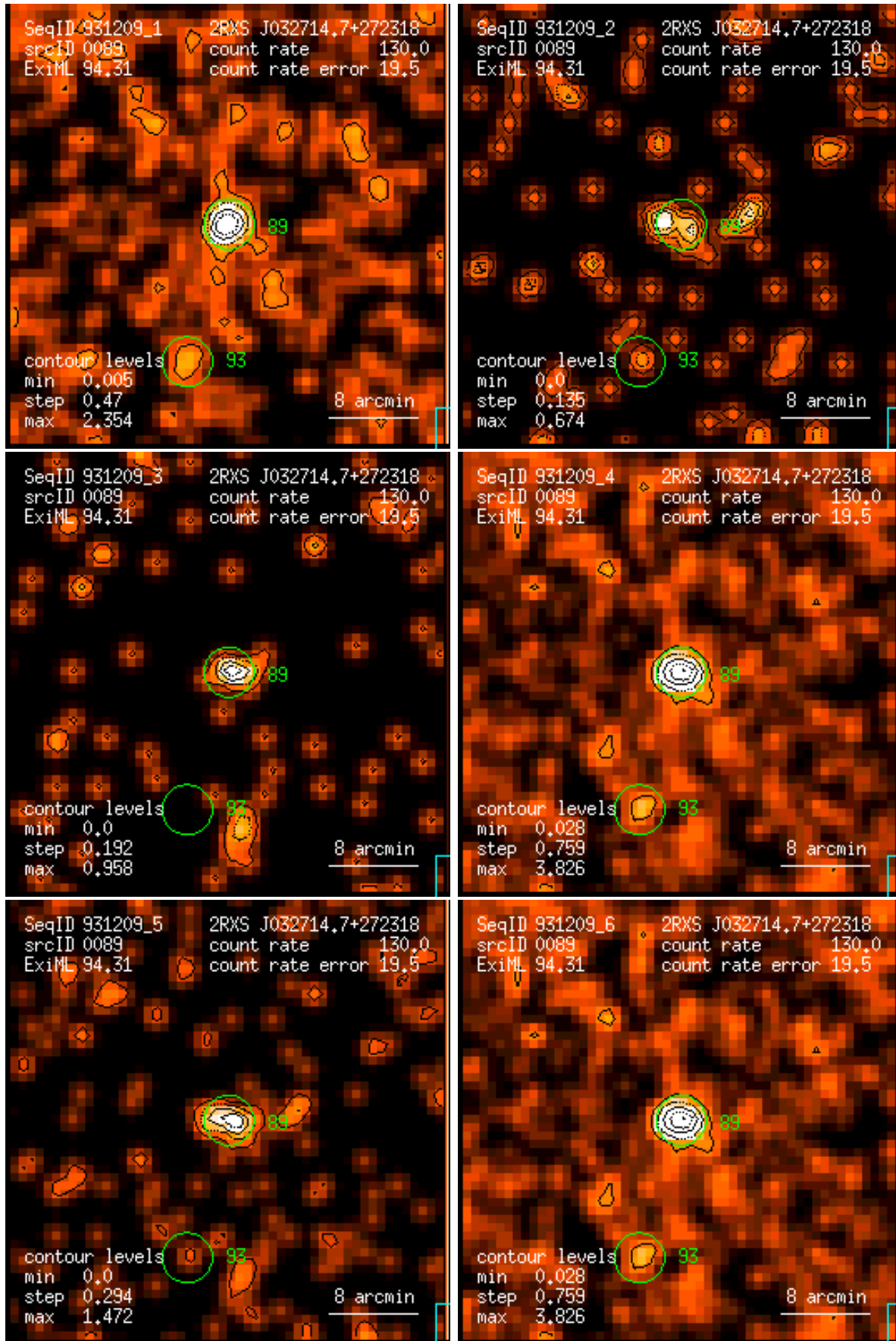
Figure 89: RASS 931209: detection 0089: band rate images, Gaussian filter: (1) PSPC channels 11 – 41, (2) 52 – 90, (3) 91 – 201, (4) 11 – 235, (5) 52 – 201, (6) 11 – 201. Broad band rates in counts/ks. Band rate contour levels in counts/ks/arcmin 2 .
