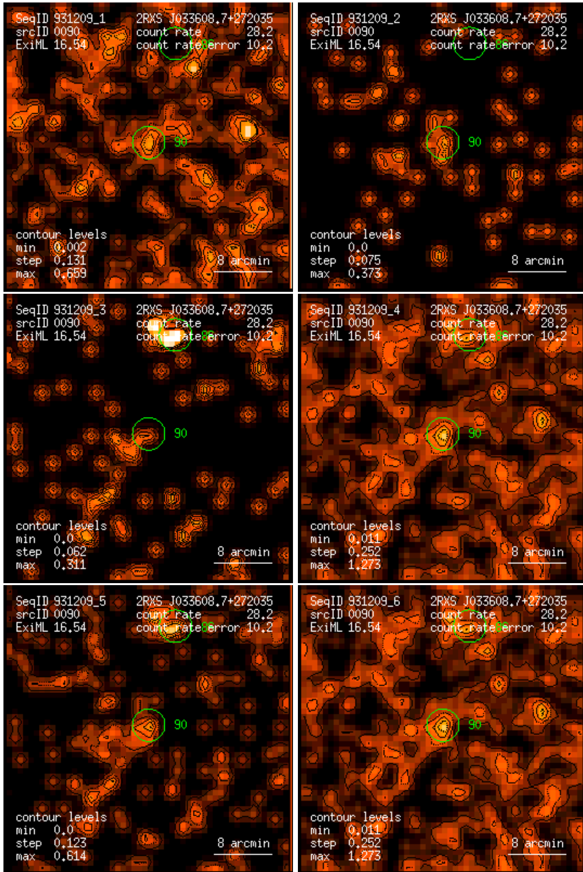
Figure 90: RASS 931209: detection 0090: band rate images, Gaussian filter: (1) PSPC channels 11 – 41, (2) 52 – 90, (3) 91 – 201, (4) 11 – 235, (5) 52 – 201, (6) 11 – 201. Broad band rates in counts/ks. Band rate contour levels in counts/ks/arcmin 2 .
