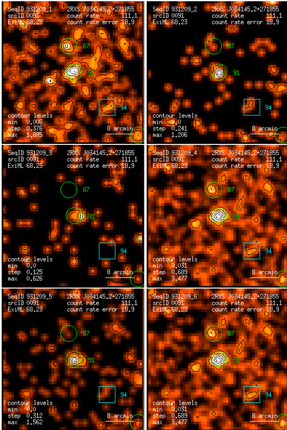
Figure 91: RASS 931209: detection 0091: band rate images, Gaussian filter: (1) PSPC channels 11 – 41, (2) 52 – 90, (3) 91 – 201, (4) 11 – 235, (5) 52 – 201, (6) 11 – 201. Broad band rates in counts/ks. Band rate contour levels in counts/ks/arcmin 2 .
