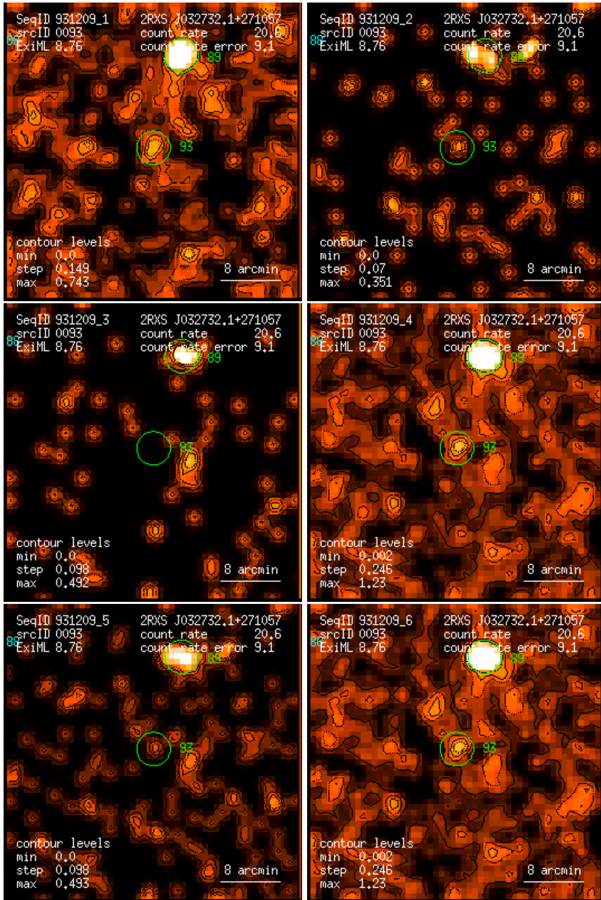
Figure 93: RASS 931209: detection 0093: band rate images, Gaussian filter: (1) PSPC channels 11 – 41, (2) 52 – 90, (3) 91 – 201, (4) 11 – 235, (5) 52 – 201, (6) 11 – 201. Broad band rates in counts/ks. Band rate contour levels in counts/ks/arcmin 2 .
