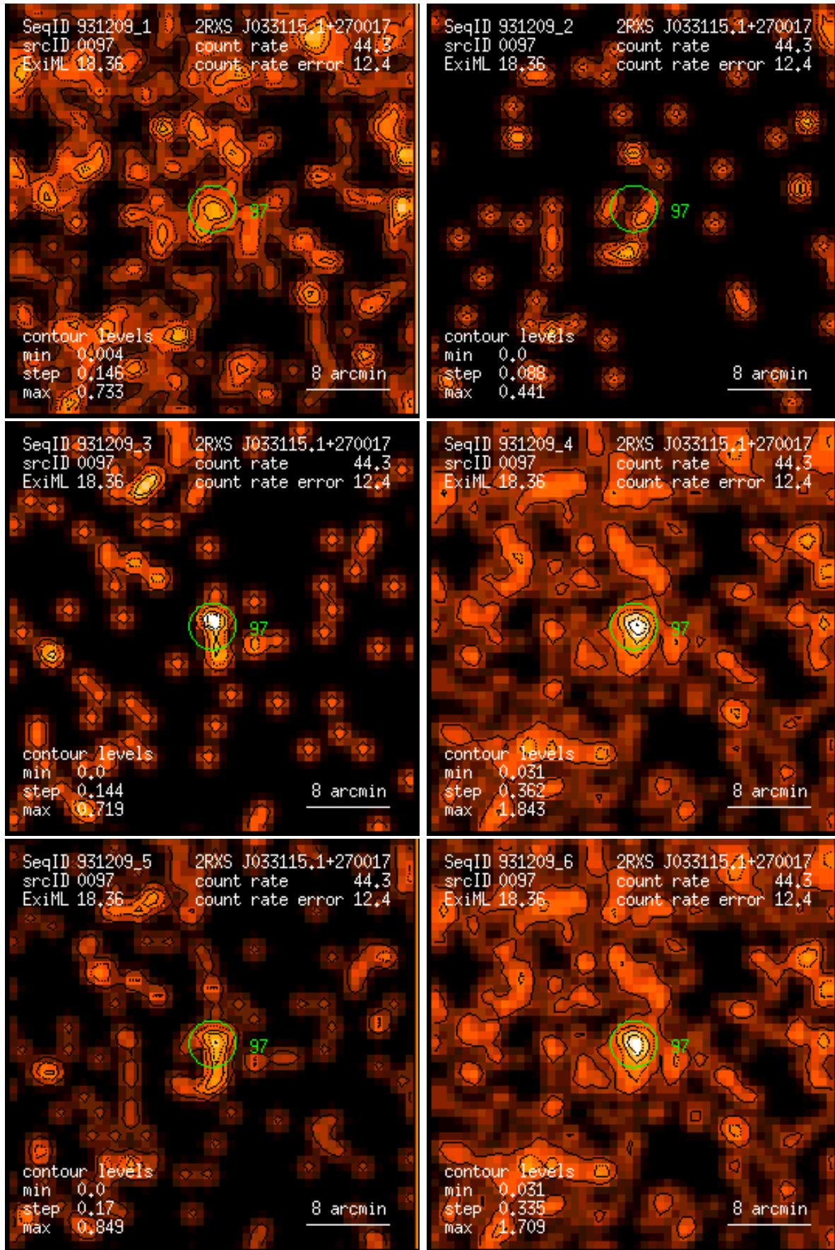
Figure 97: RASS 931209: detection 0097: band rate images, Gaussian filter: (1) PSPC channels 11 – 41, (2) 52 – 90, (3) 91 – 201, (4) 11 – 235, (5) 52 – 201, (6) 11 – 201. Broad band rates in counts/ks. Band rate contour levels in counts/ks/arcmin 2 .
