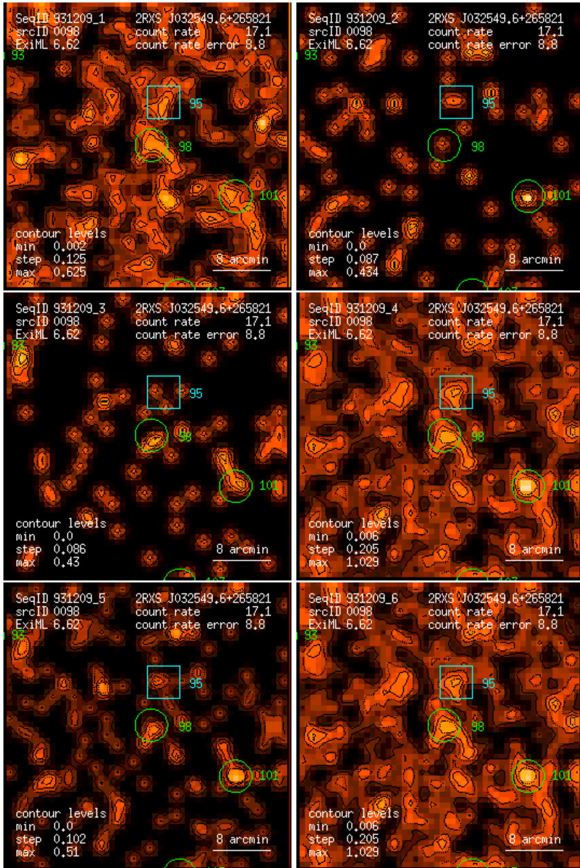
Figure 98: RASS 931209: detection 0098: band rate images, Gaussian filter: (1) PSPC channels 11 – 41, (2) 52 – 90, (3) 91 – 201, (4) 11 – 235, (5) 52 – 201, (6) 11 – 201. Broad band rates in counts/ks. Band rate contour levels in counts/ks/arcmin 2 .
