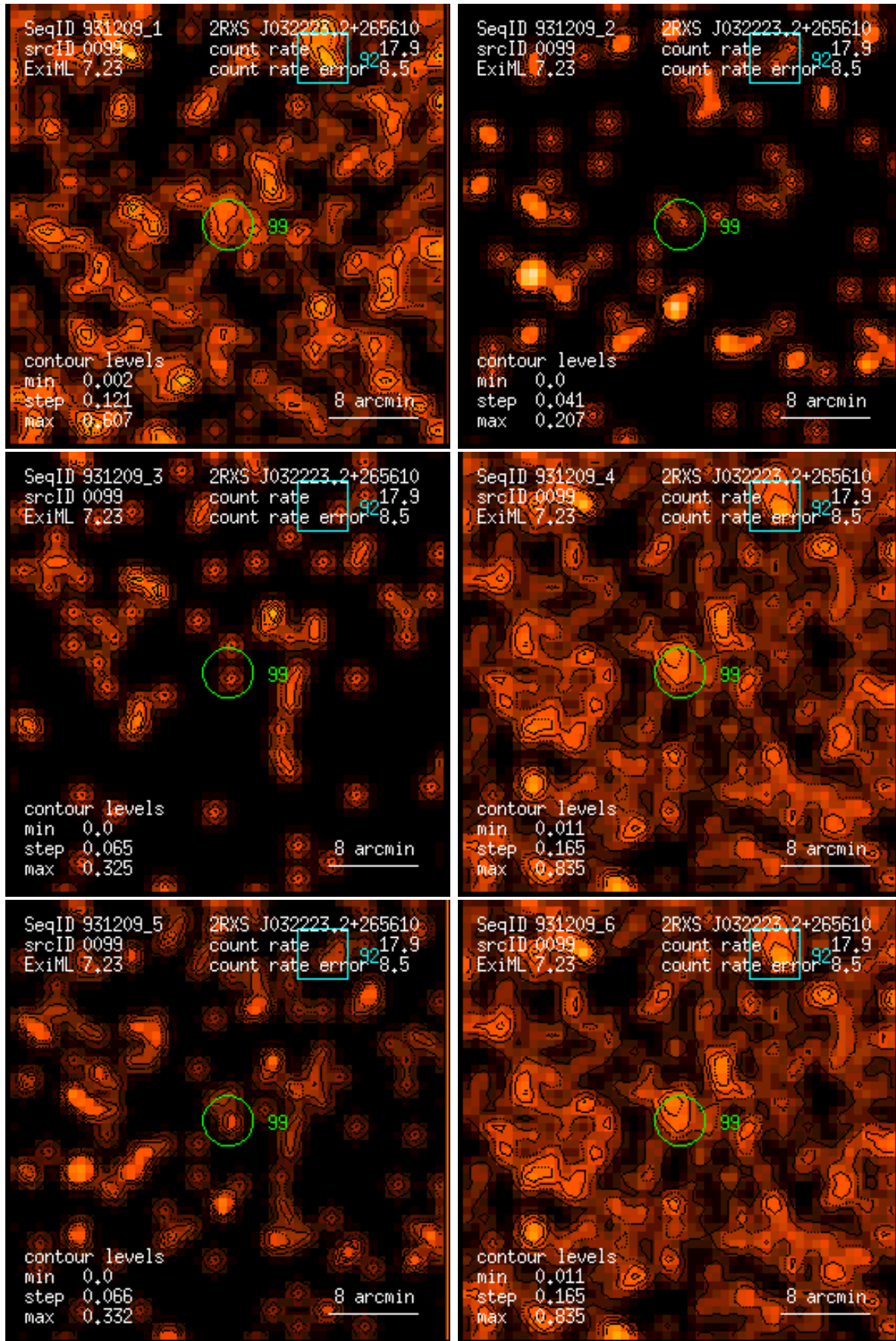
Figure 99: RASS 931209: detection 0099: band rate images, Gaussian filter: (1) PSPC channels 11 – 41, (2) 52 – 90, (3) 91 – 201, (4) 11 – 235, (5) 52 – 201, (6) 11 – 201. Broad band rates in counts/ks. Band rate contour levels in counts/ks/arcmin 2 .
