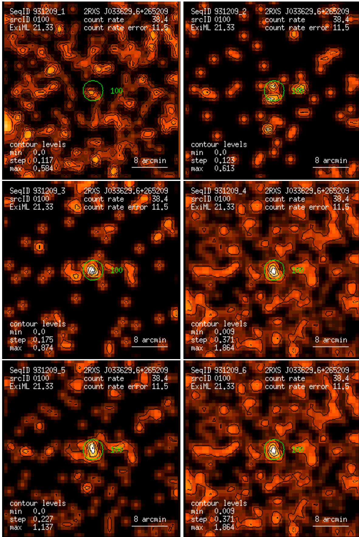
Figure 100: RASS 931209: detection 0100: band rate images, Gaussian filter: (1) PSPC channels 11 – 41, (2) 52 – 90, (3) 91 – 201, (4) 11 – 235, (5) 52 – 201, (6) 11 – 201. Broad band rates in counts/ks. Band rate contour levels in counts/ks/arcmin 2 .
