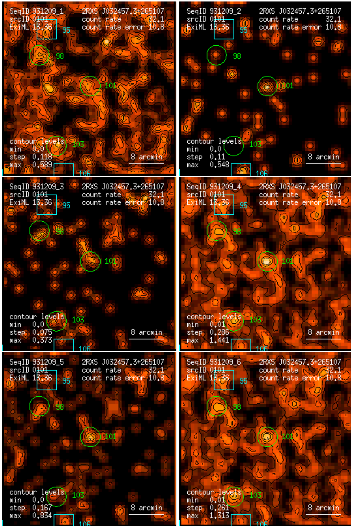
Figure 101: RASS 931209: detection 0101: band rate images, Gaussian filter: (1) PSPC channels 11 – 41, (2) 52 – 90, (3) 91 – 201, (4) 11 – 235, (5) 52 – 201, (6) 11 – 201. Broad band rates in counts/ks. Band rate contour levels in counts/ks/arcmin 2 .
