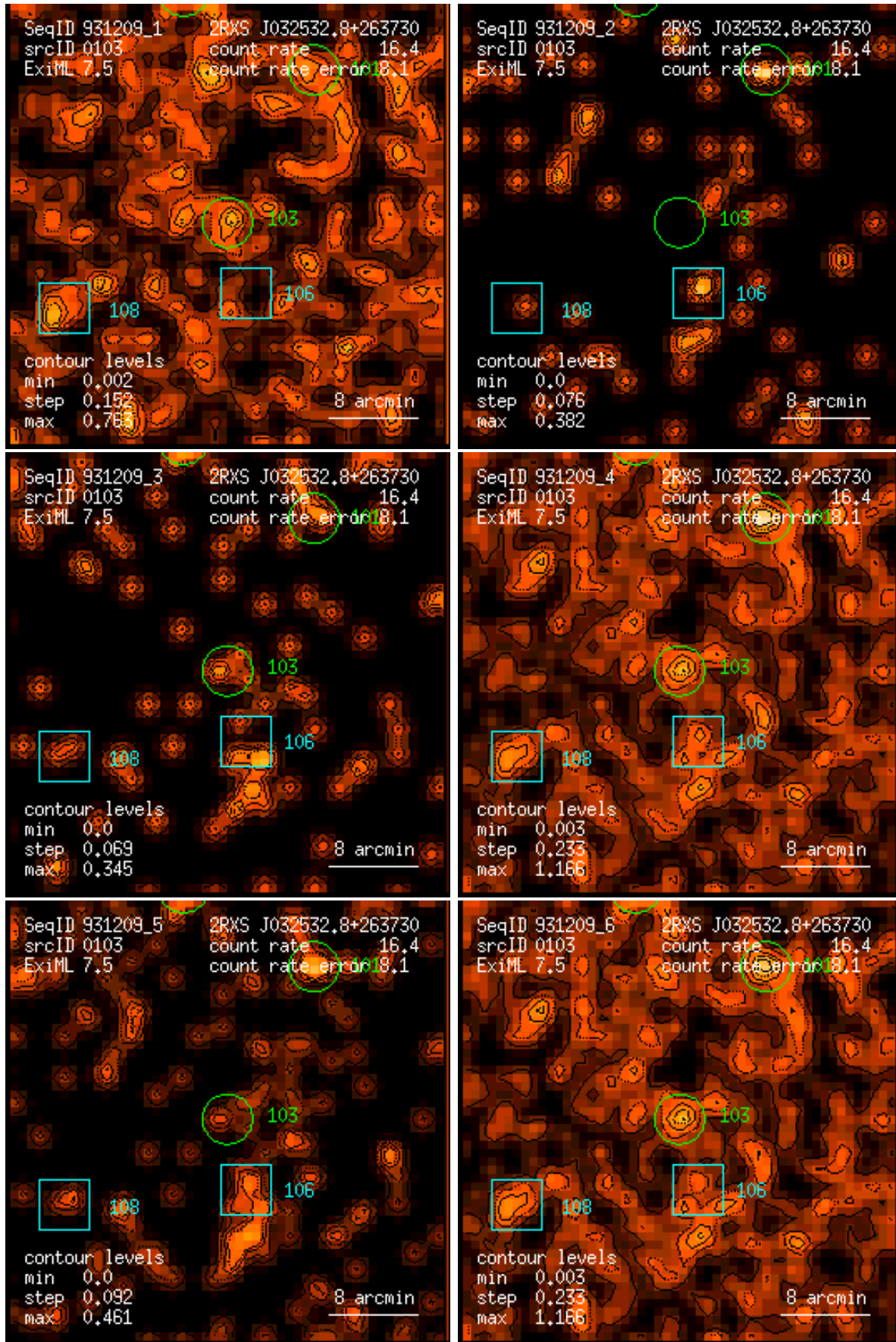
Figure 103: RASS 931209: detection 0103: band rate images, Gaussian filter: (1) PSPC channels 11 – 41, (2) 52 – 90, (3) 91 – 201, (4) 11 – 235, (5) 52 – 201, (6) 11 – 201. Broad band rates in counts/ks. Band rate contour levels in counts/ks/arcmin 2 .
