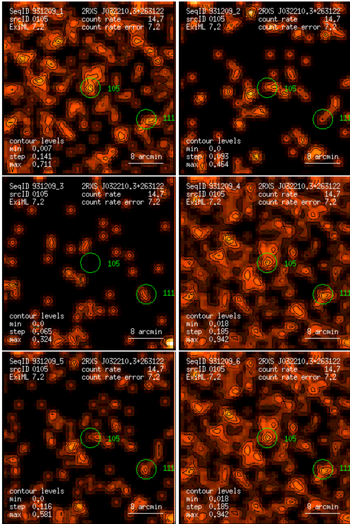
Figure 105: RASS 931209: detection 0105: band rate images, Gaussian filter: (1) PSPC channels 11 – 41, (2) 52 – 90, (3) 91 – 201, (4) 11 – 235, (5) 52 – 201, (6) 11 – 201. Broad band rates in counts/ks. Band rate contour levels in counts/ks/arcmin 2 .
