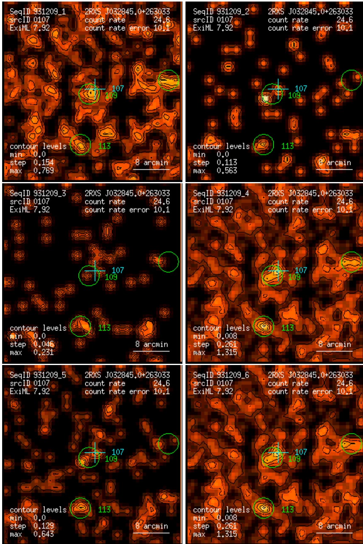
Figure 107: RASS 931209: detection 0107: band rate images, Gaussian filter: (1) PSPC channels 11 – 41, (2) 52 – 90, (3) 91 – 201, (4) 11 – 235, (5) 52 – 201, (6) 11 – 201. Broad band rates in counts/ks. Band rate contour levels in counts/ks/arcmin 2 .
