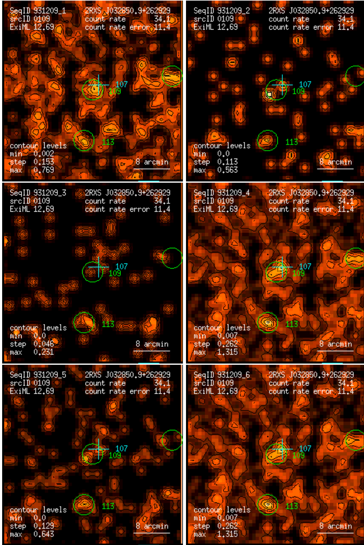
Figure 109: RASS 931209: detection 0109: band rate images, Gaussian filter: (1) PSPC channels 11 – 41, (2) 52 – 90, (3) 91 – 201, (4) 11 – 235, (5) 52 – 201, (6) 11 – 201. Broad band rates in counts/ks. Band rate contour levels in counts/ks/arcmin 2 .
