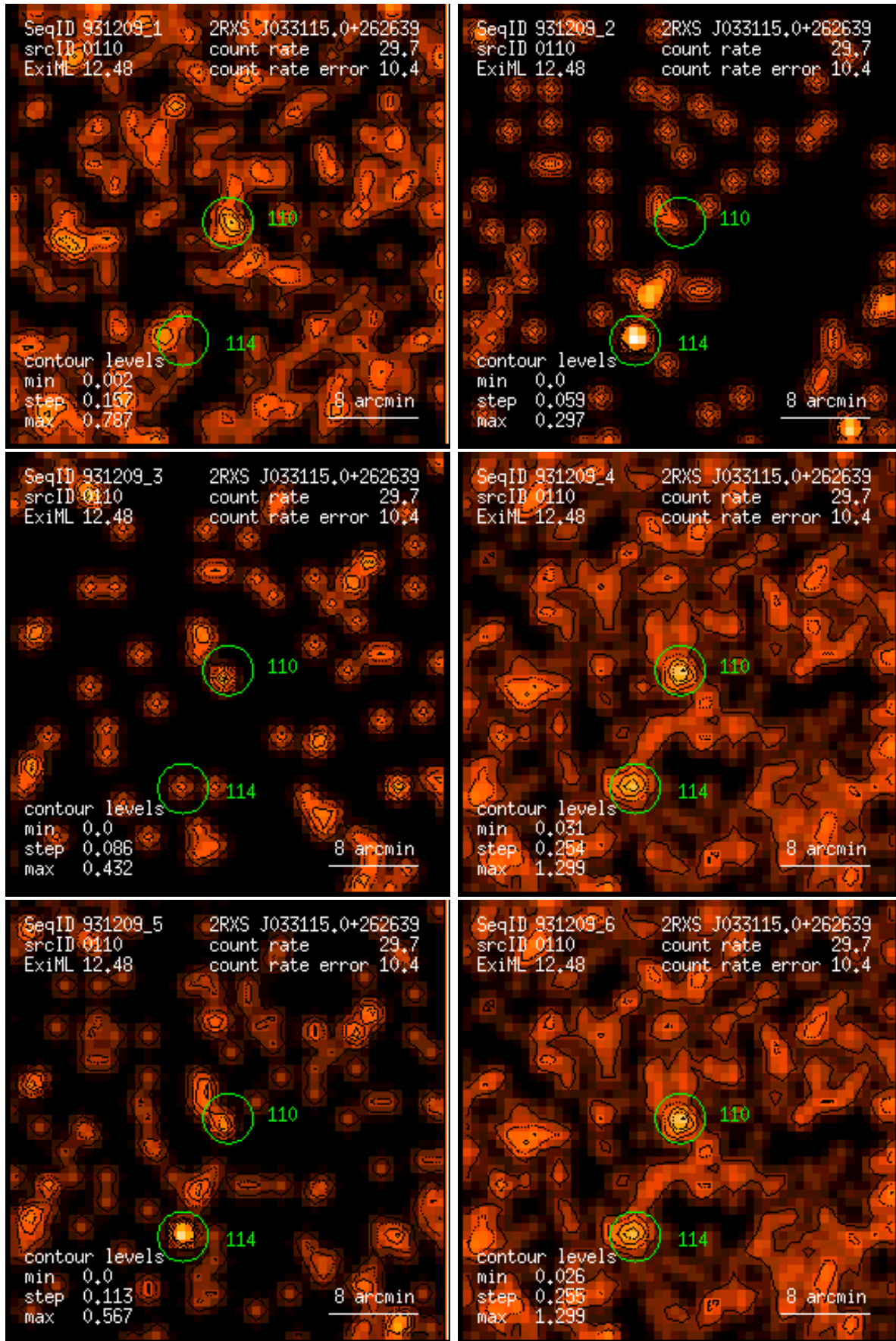
Figure 110: RASS 931209: detection 0110: band rate images, Gaussian filter: (1) PSPC channels 11 – 41, (2) 52 – 90, (3) 91 – 201, (4) 11 – 235, (5) 52 – 201, (6) 11 – 201. Broad band rates in counts/ks. Band rate contour levels in counts/ks/arcmin 2 .
