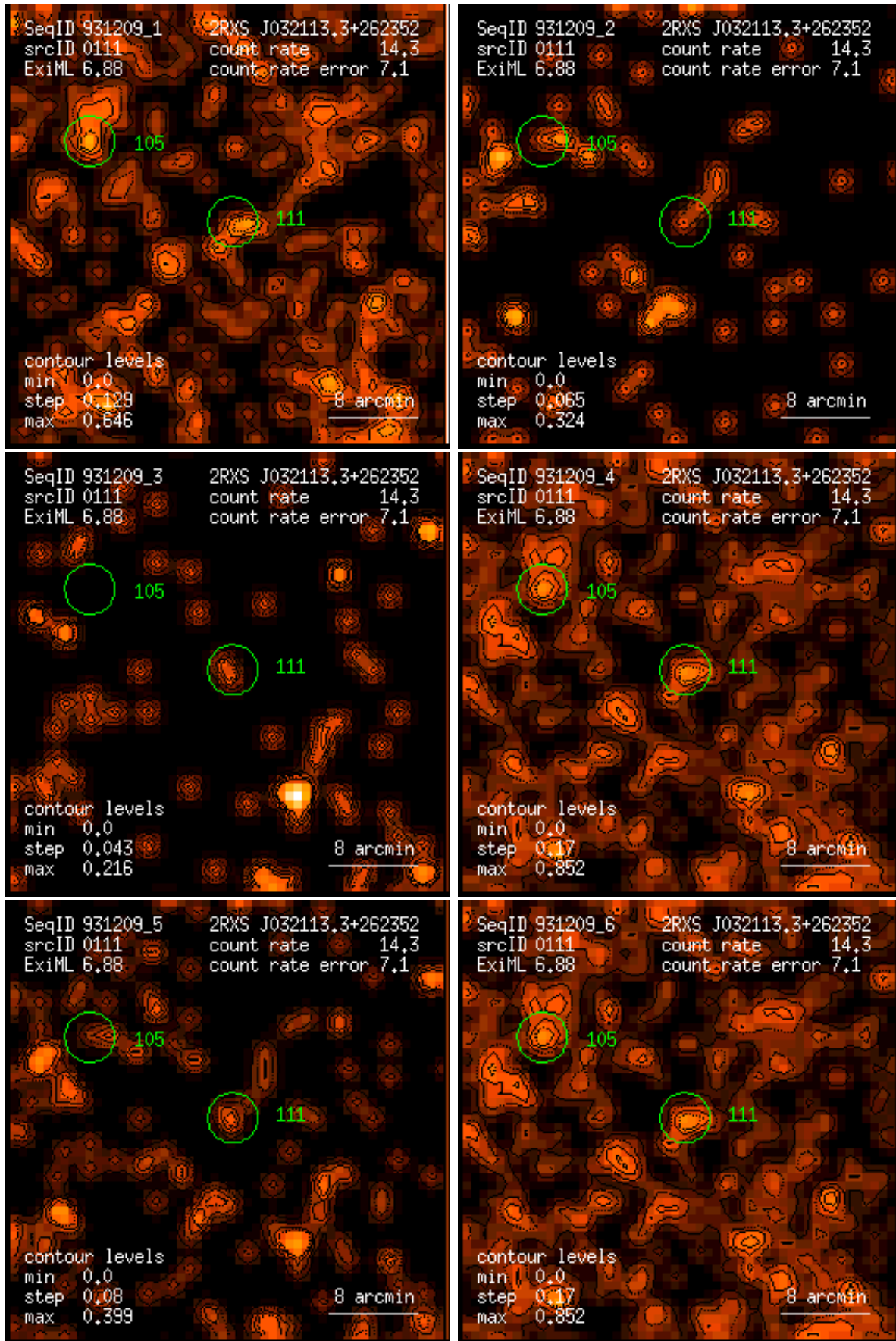
Figure 111: RASS 931209: detection 0111: band rate images, Gaussian filter: (1) PSPC channels 11 – 41, (2) 52 – 90, (3) 91 – 201, (4) 11 – 235, (5) 52 – 201, (6) 11 – 201. Broad band rates in counts/ks. Band rate contour levels in counts/ks/arcmin 2 .
