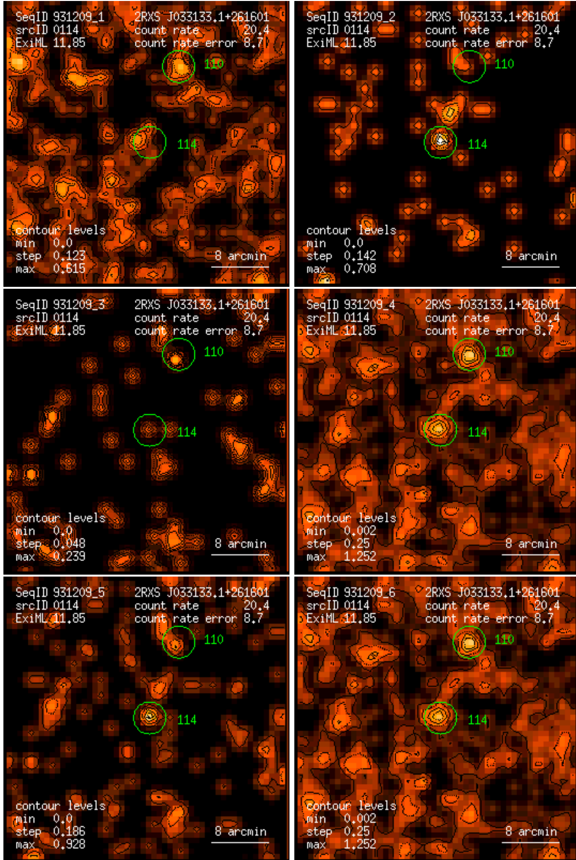
Figure 114: RASS 931209: detection 0114: band rate images, Gaussian filter: (1) PSPC channels 11 – 41, (2) 52 – 90, (3) 91 – 201, (4) 11 – 235, (5) 52 – 201, (6) 11 – 201. Broad band rates in counts/ks. Band rate contour levels in counts/ks/arcmin 2 .
