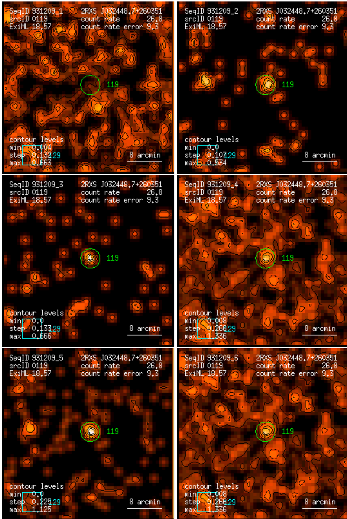
Figure 119: RASS 931209: detection 0119: band rate images, Gaussian filter: (1) PSPC channels 11 – 41, (2) 52 – 90, (3) 91 – 201, (4) 11 – 235, (5) 52 – 201, (6) 11 – 201. Broad band rates in counts/ks. Band rate contour levels in counts/ks/arcmin 2 .
