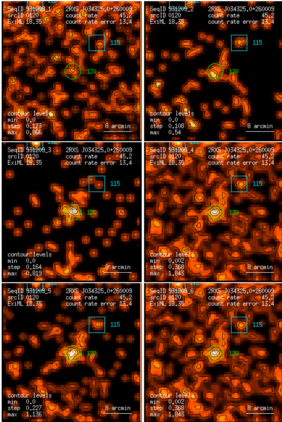
Figure 120: RASS 931209: detection 0120: band rate images, Gaussian filter: (1) PSPC channels 11 – 41, (2) 52 – 90, (3) 91 – 201, (4) 11 – 235, (5) 52 – 201, (6) 11 – 201. Broad band rates in counts/ks. Band rate contour levels in counts/ks/arcmin 2 .
