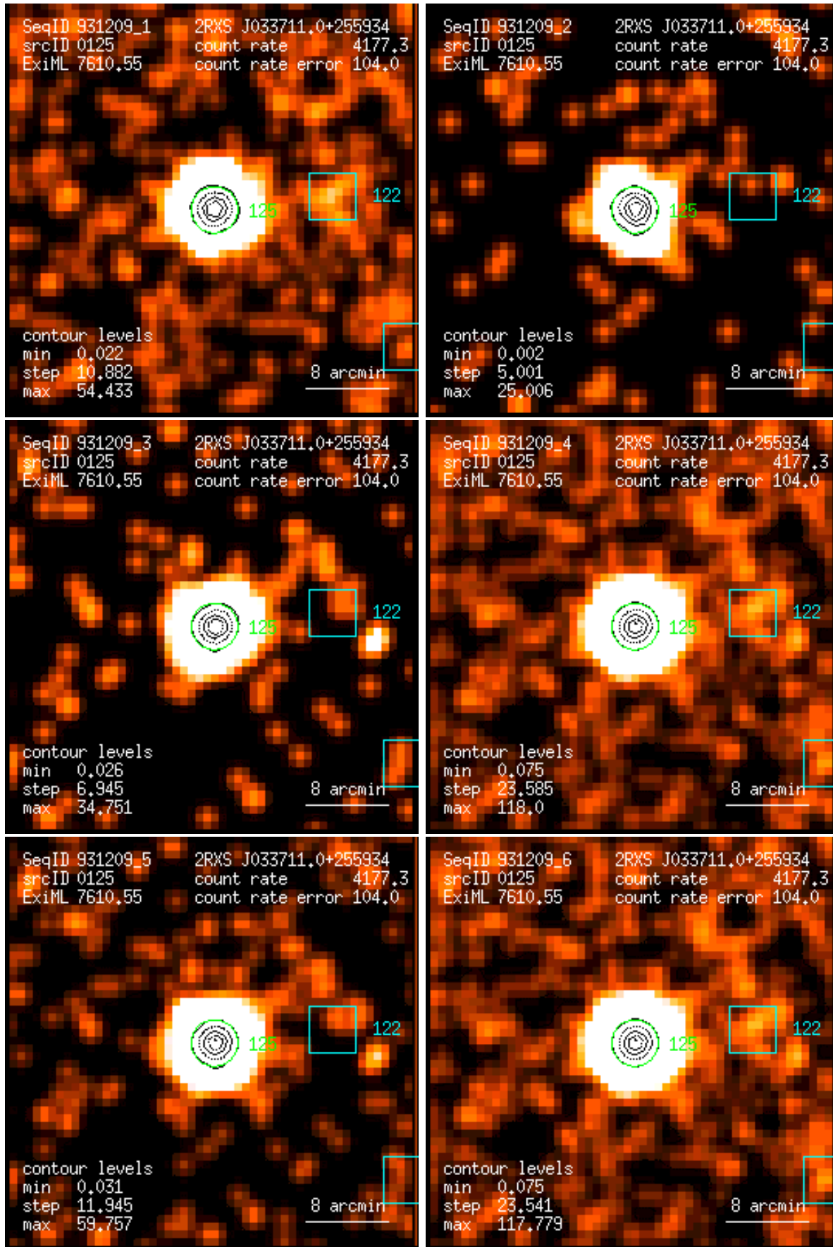
Figure 125: RASS 931209: detection 0125: band rate images, Gaussian filter: (1) PSPC channels 11 – 41, (2) 52 – 90, (3) 91 – 201, (4) 11 – 235, (5) 52 – 201, (6) 11 – 201. Broad band rates in counts/ks. Band rate contour levels in counts/ks/arcmin 2 .
