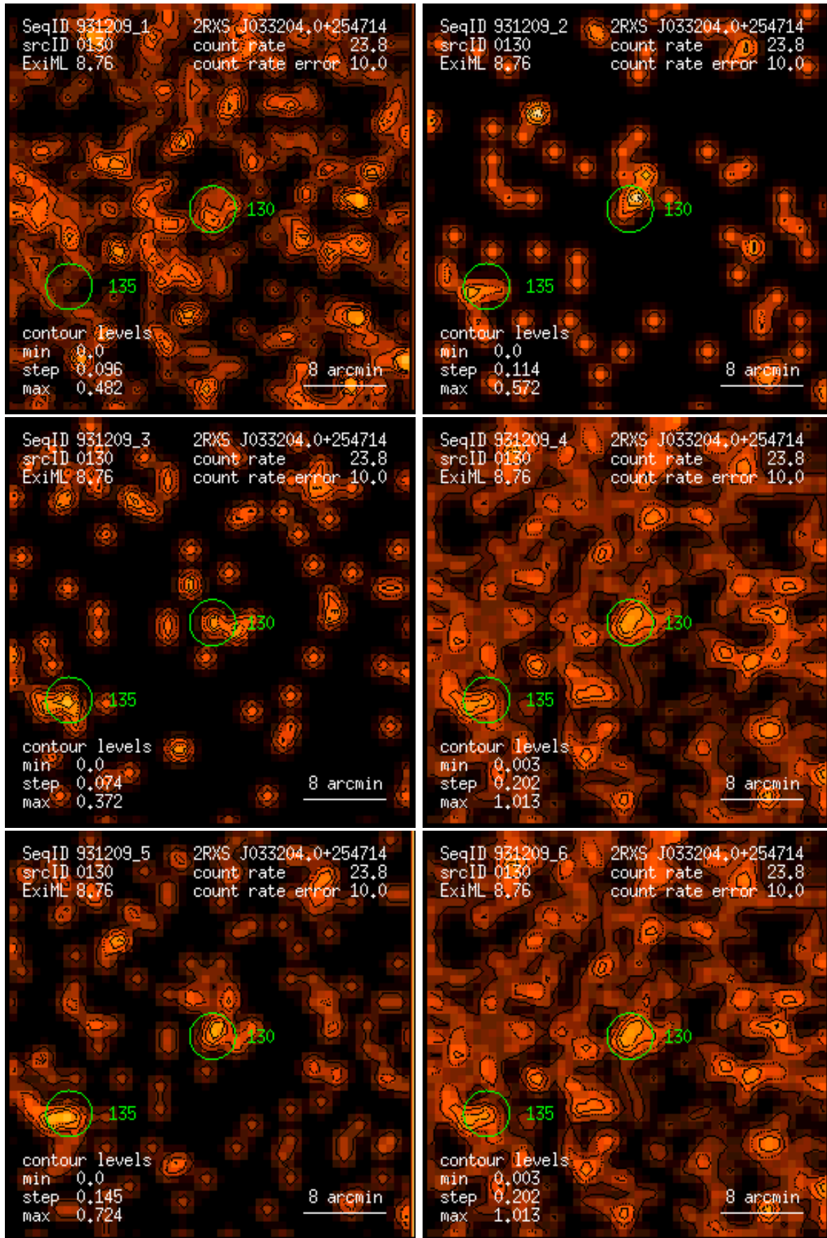
Figure 130: RASS 931209: detection 0130: band rate images, Gaussian filter: (1) PSPC channels 11 – 41, (2) 52 – 90, (3) 91 – 201, (4) 11 – 235, (5) 52 – 201, (6) 11 – 201. Broad band rates in counts/ks. Band rate contour levels in counts/ks/arcmin 2 .
