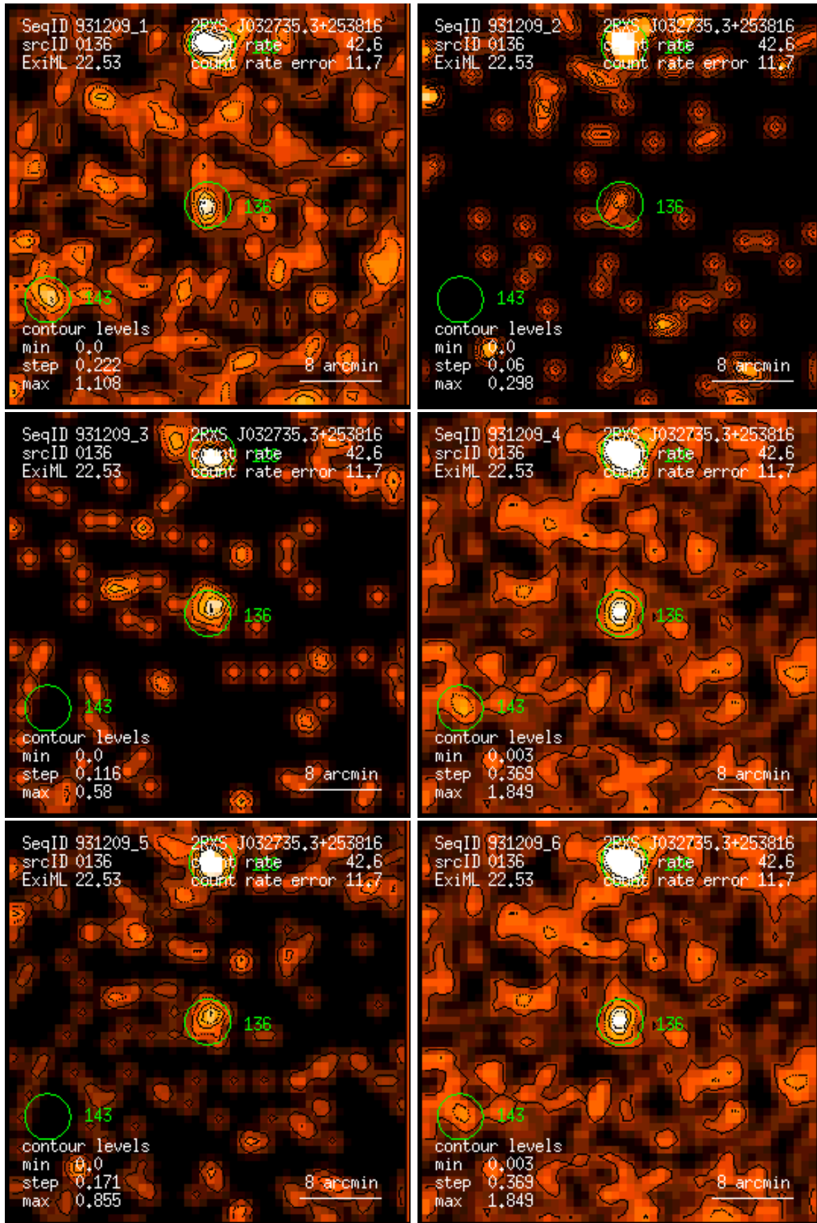
Figure 136: RASS 931209: detection 0136: band rate images, Gaussian filter: (1) PSPC channels 11 – 41, (2) 52 – 90, (3) 91 – 201, (4) 11 – 235, (5) 52 – 201, (6) 11 – 201. Broad band rates in counts/ks. Band rate contour levels in counts/ks/arcmin 2 .
