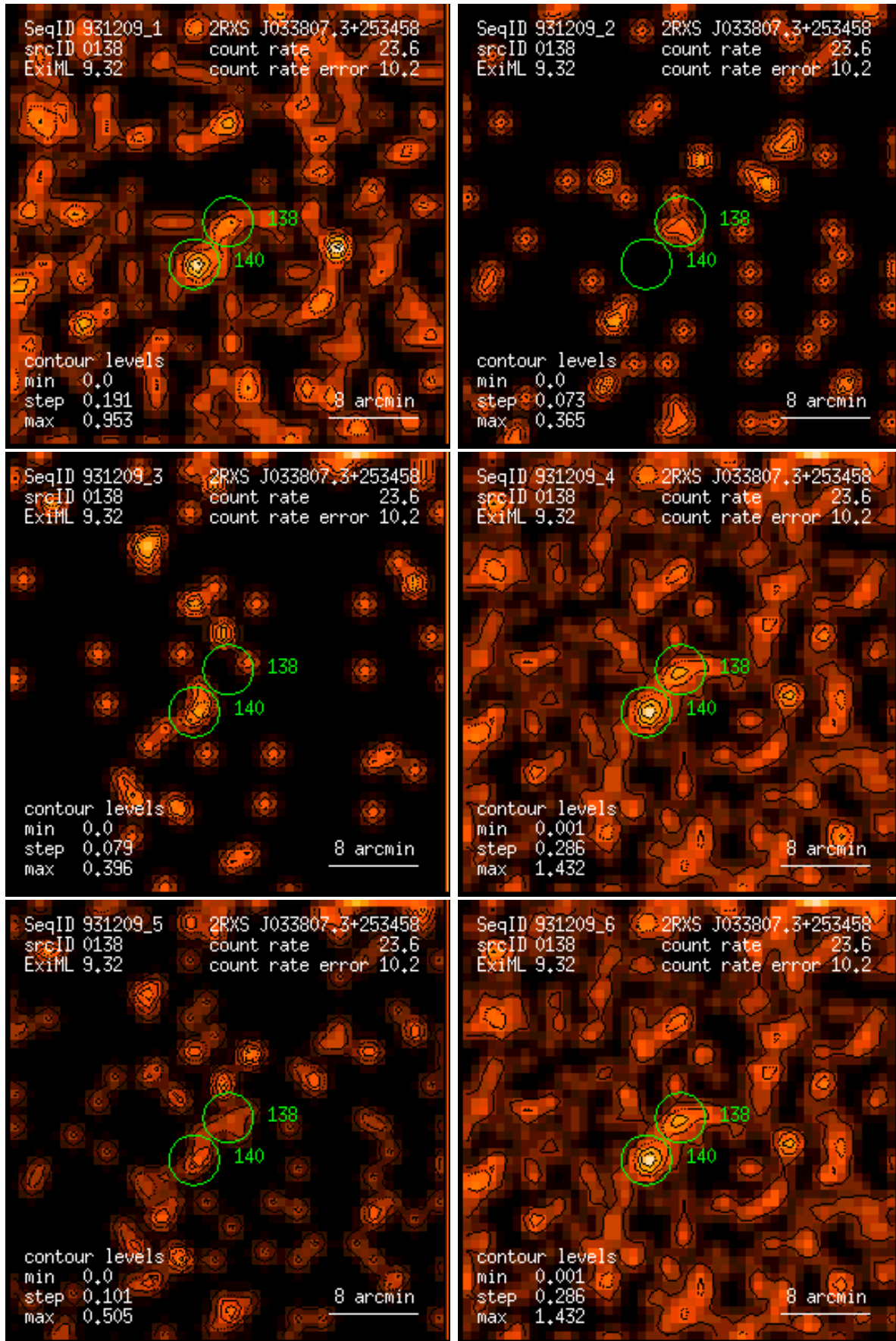
Figure 138: RASS 931209: detection 0138: band rate images, Gaussian filter: (1) PSPC channels 11 – 41, (2) 52 – 90, (3) 91 – 201, (4) 11 – 235, (5) 52 – 201, (6) 11 – 201. Broad band rates in counts/ks. Band rate contour levels in counts/ks/arcmin 2 .
