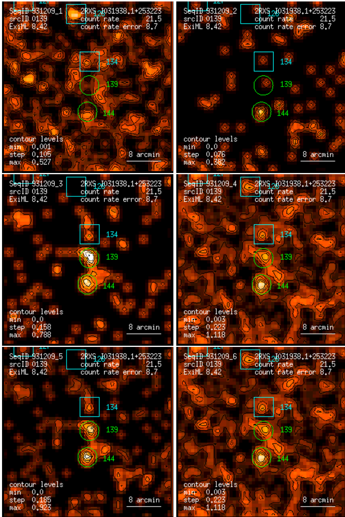
Figure 139: RASS 931209: detection 0139: band rate images, Gaussian filter: (1) PSPC channels 11 – 41, (2) 52 – 90, (3) 91 – 201, (4) 11 – 235, (5) 52 – 201, (6) 11 – 201. Broad band rates in counts/ks. Band rate contour levels in counts/ks/arcmin 2 .
